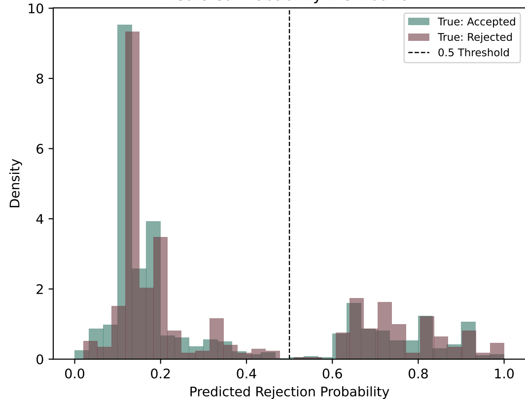
Predicted Probability Distribution
