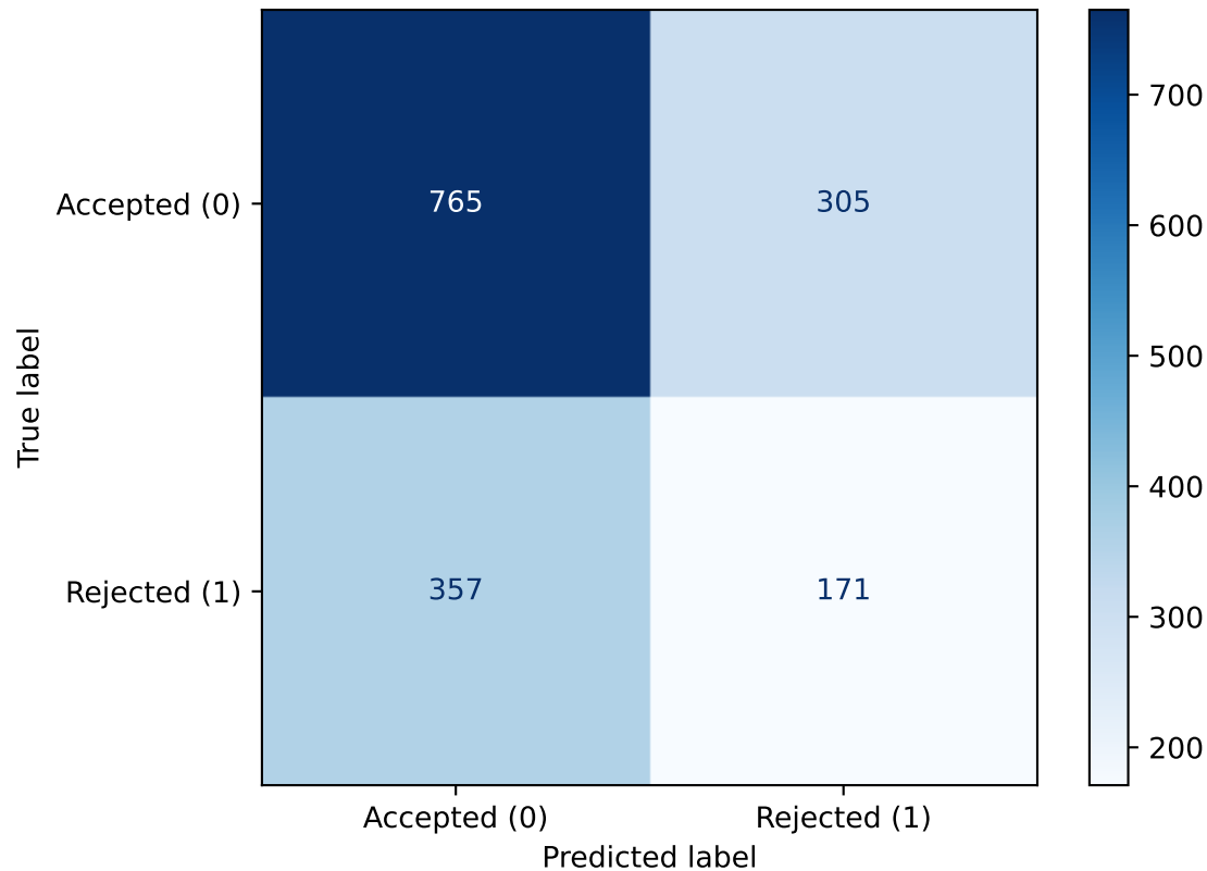
Confusion Matrix
