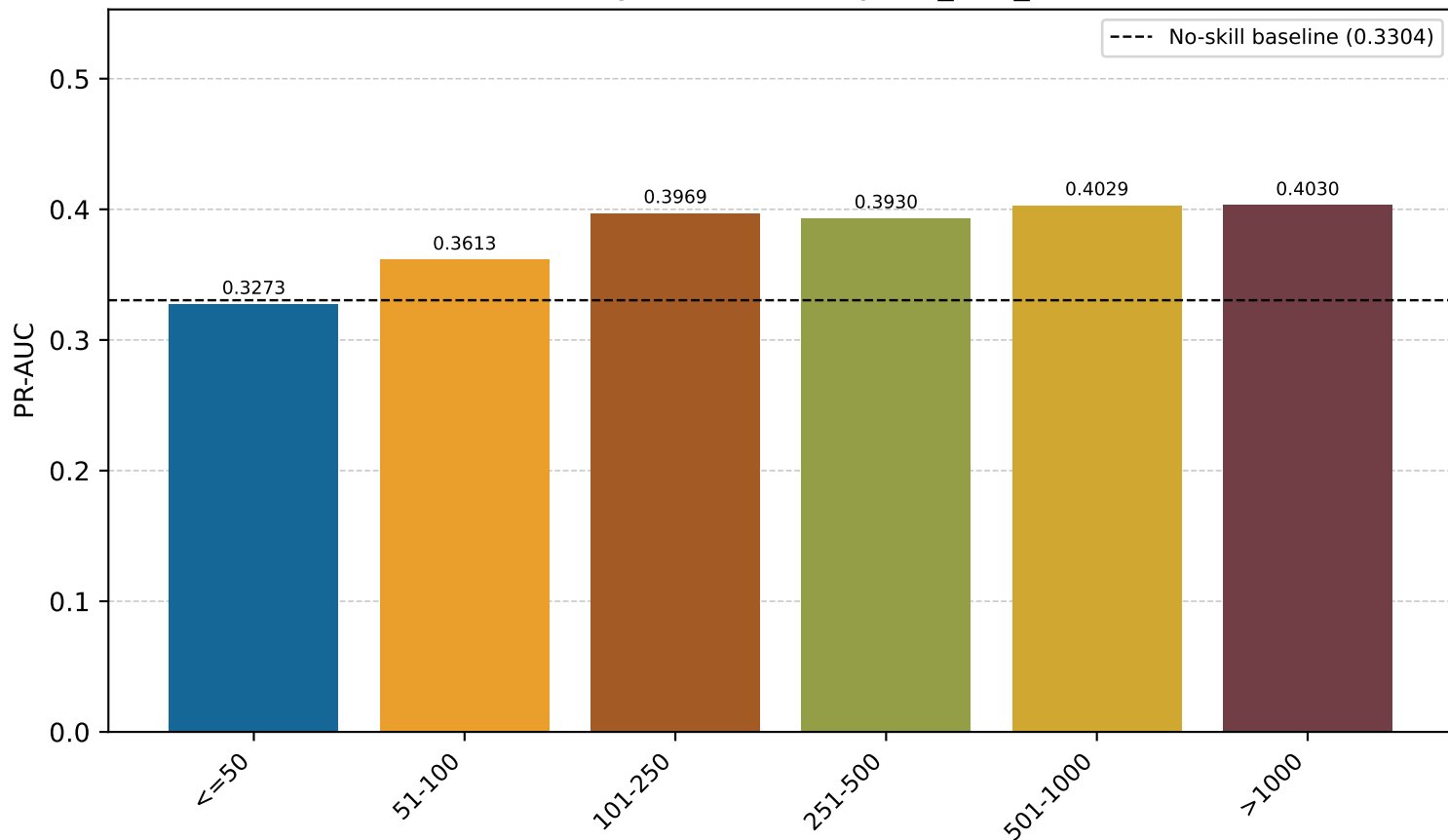
QwQ Reasoning LLM PR-AUC by diff_size_bin — Val
