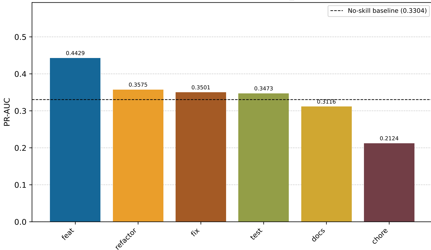
QwQ Reasoning LLM PR-AUC by task_type — Val
