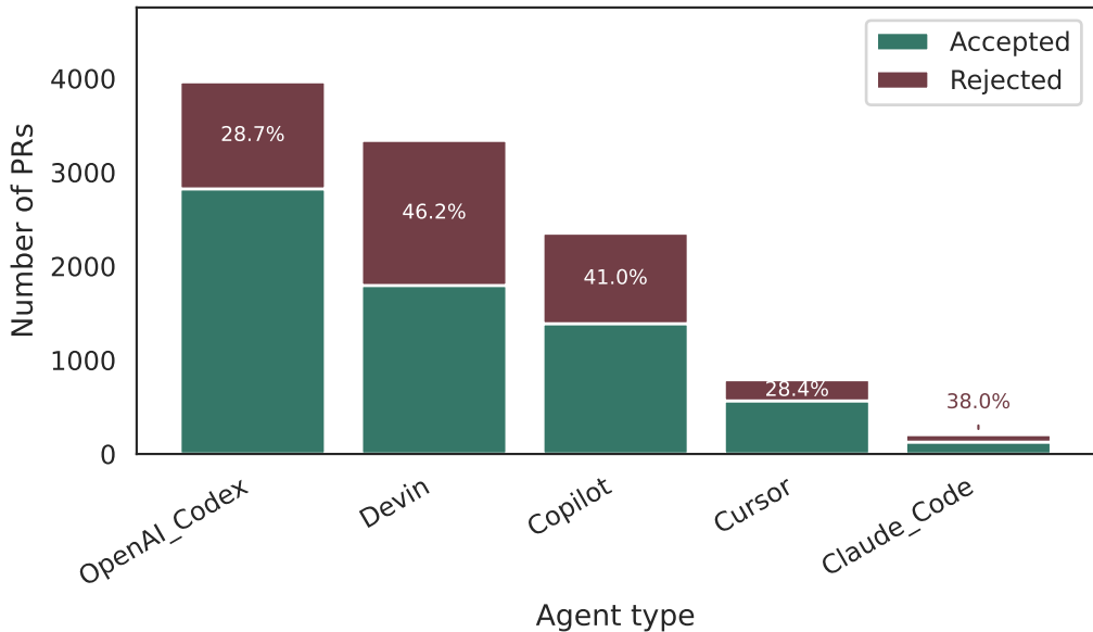
PR count by agent type
