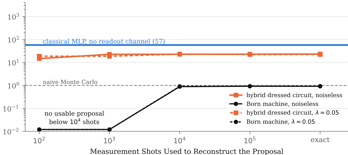
Variance Reduction Factor
