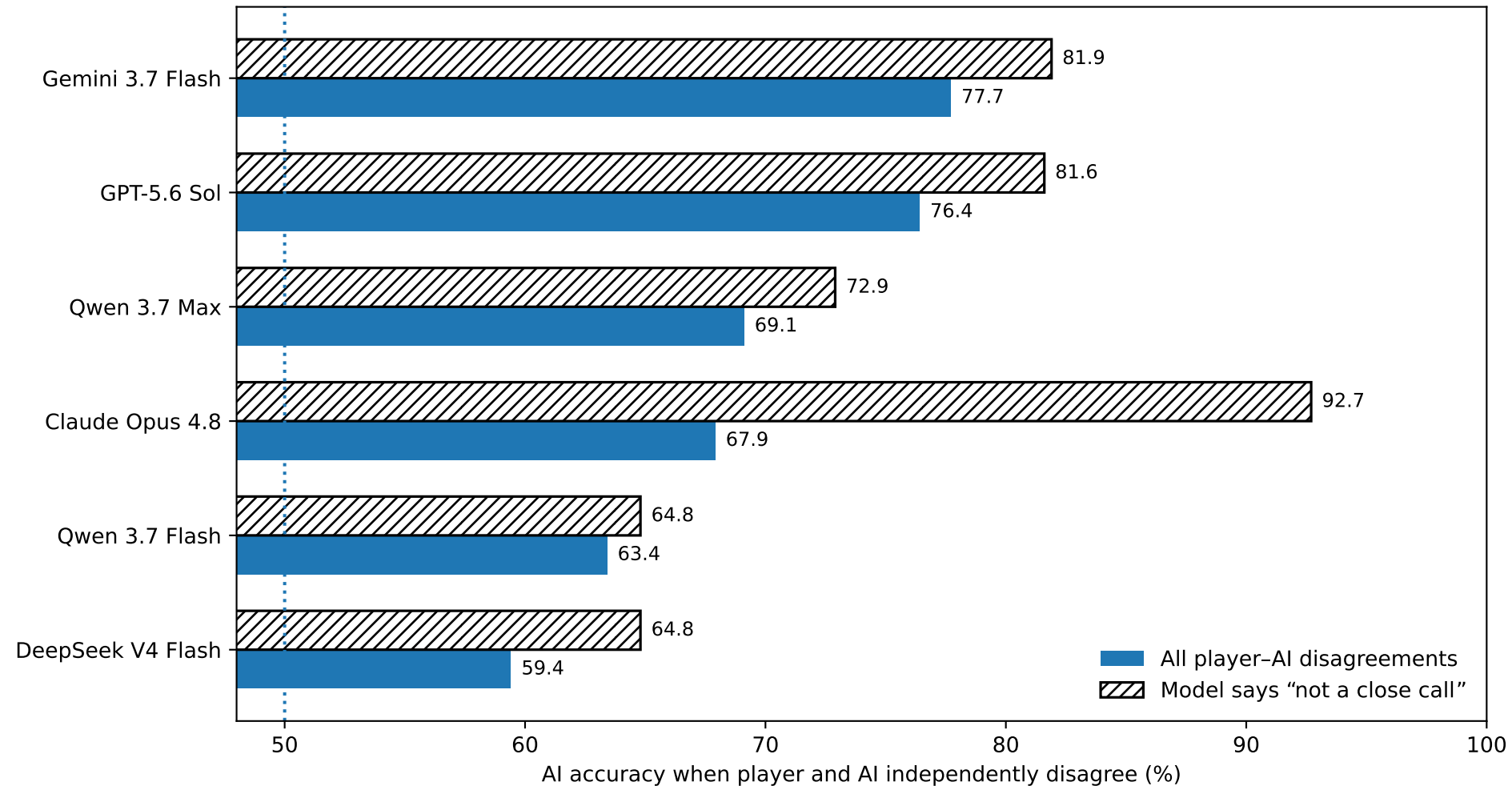
Model uncertainty helps identify higher-value disagreement cases
