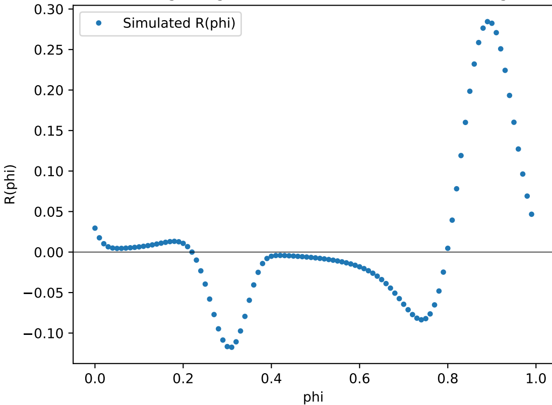
FitzHugh-Nagumo: \delta = 10^{-3} , shift in 5th crossing
