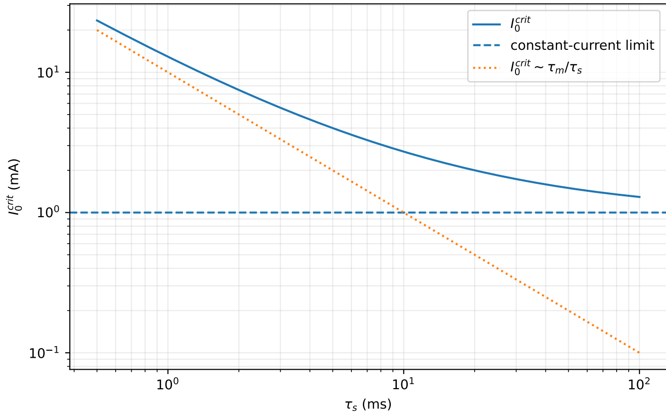
Critical synaptic amplitude, \tau_m = 10 ms, R = 1\ \Omega
