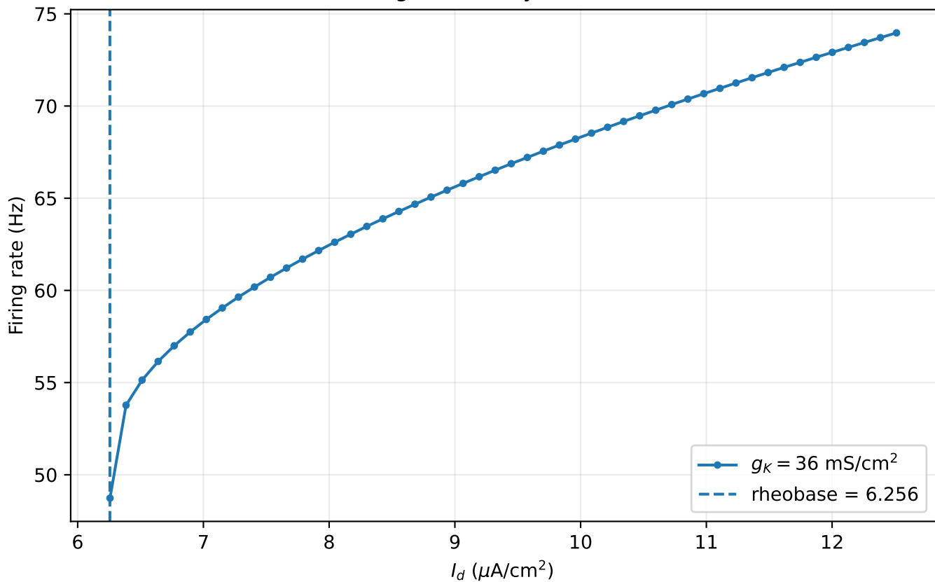
Hodgkin--Huxley f - I curve
