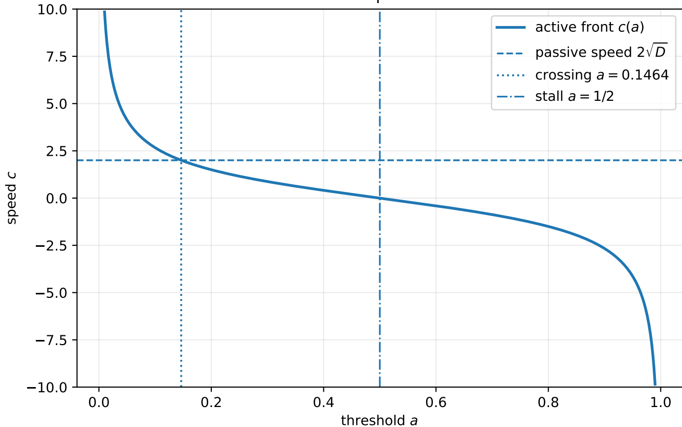
Active front speed for D = 1
