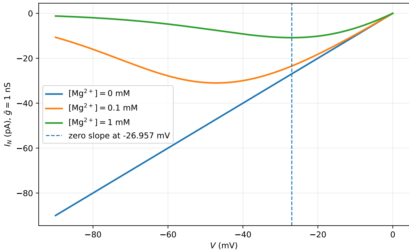
Voltage-dependent NMDA current, E_N = 0 mV, V_0 = 16.13 mV
