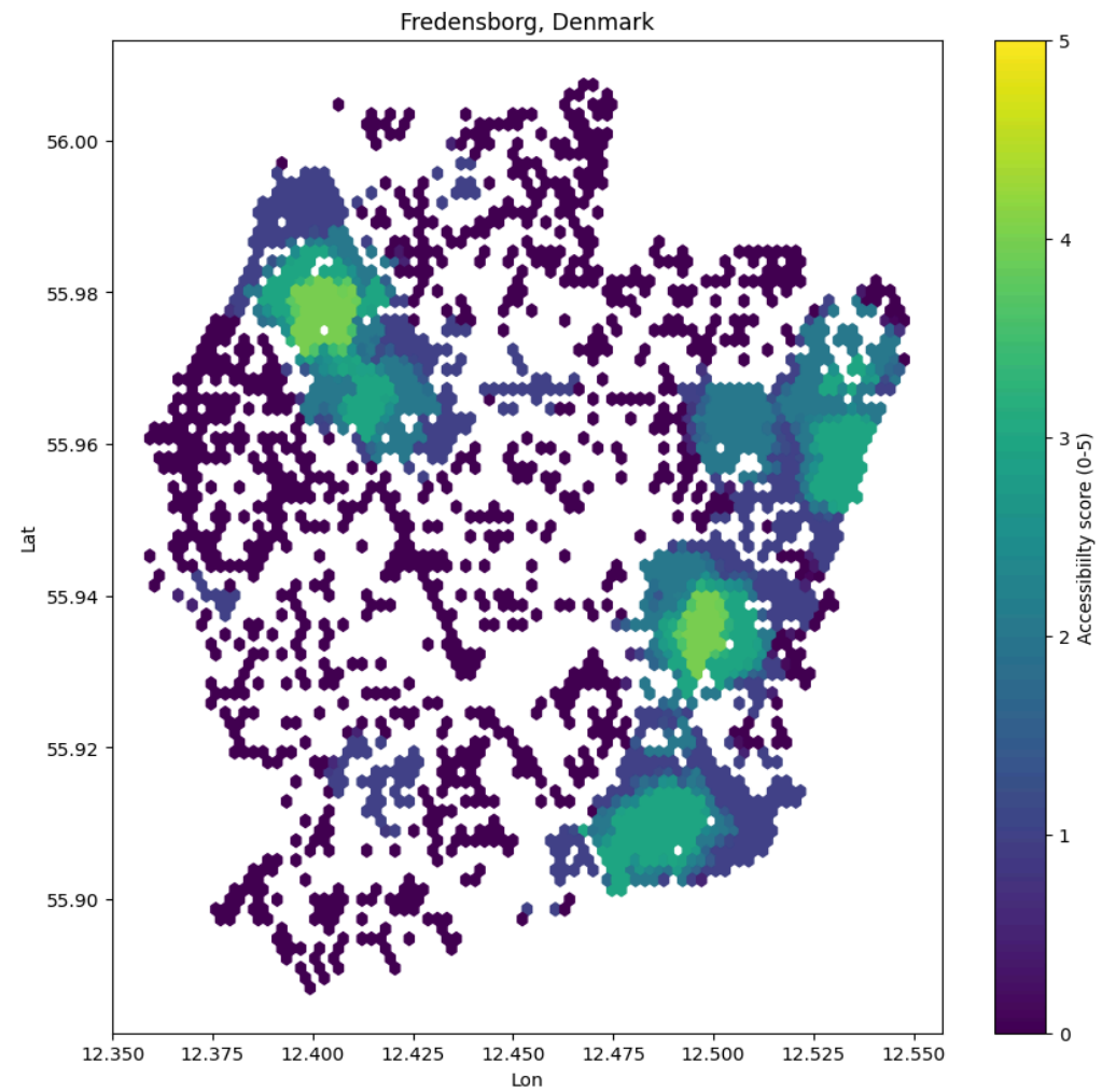
Figure 1: Example of accessibility scoring a small city in Denmark
