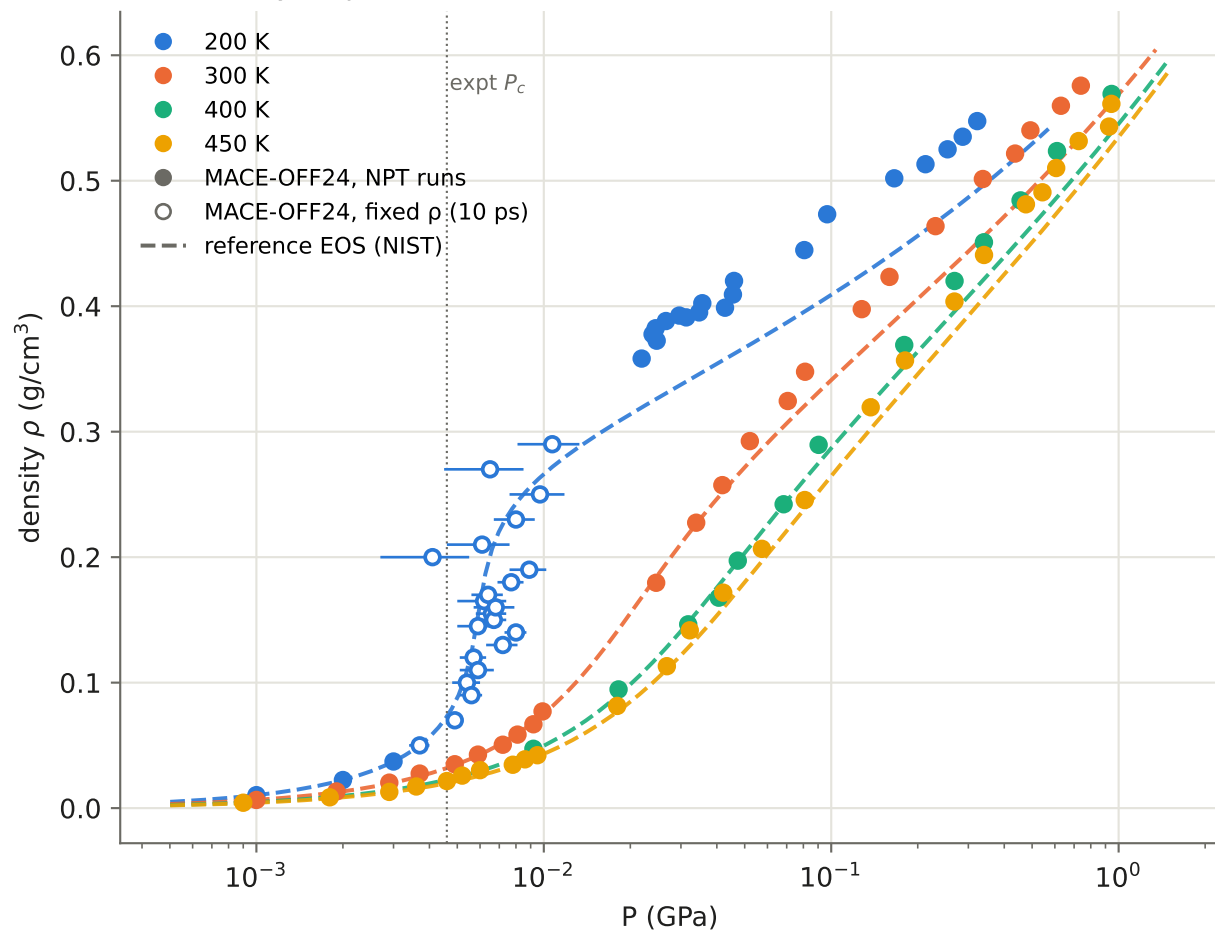
CH 4 density vs pressure
