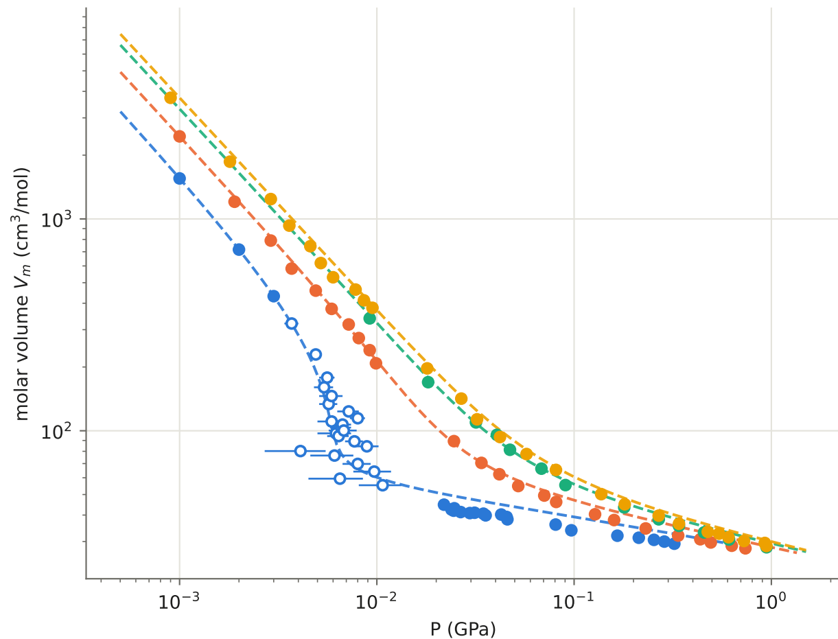
CH 4 P-V: MACE-OFF24 vs reference EOS
