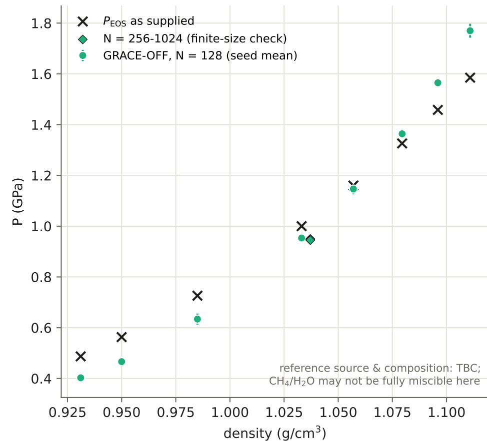
(c) CH 4 /H 2 O mixture, ~400 K
