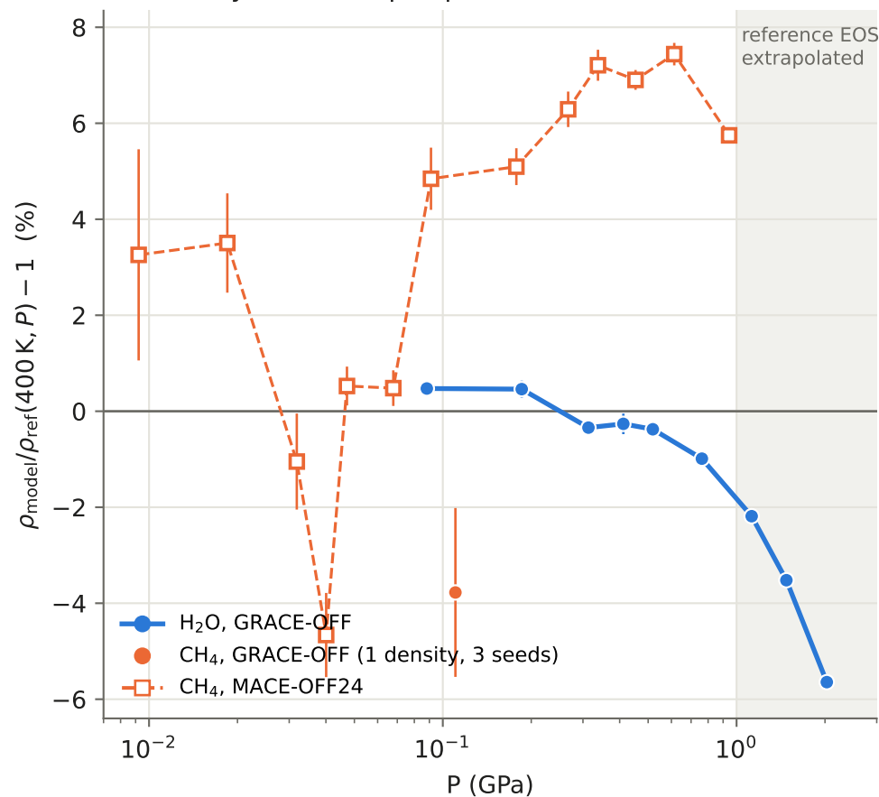
(b) density error at equal pressure, 400 K
