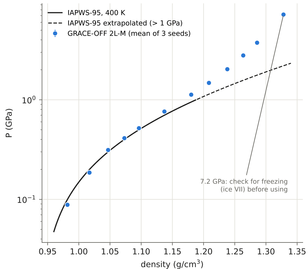
(a) H 2 O at 400 K
