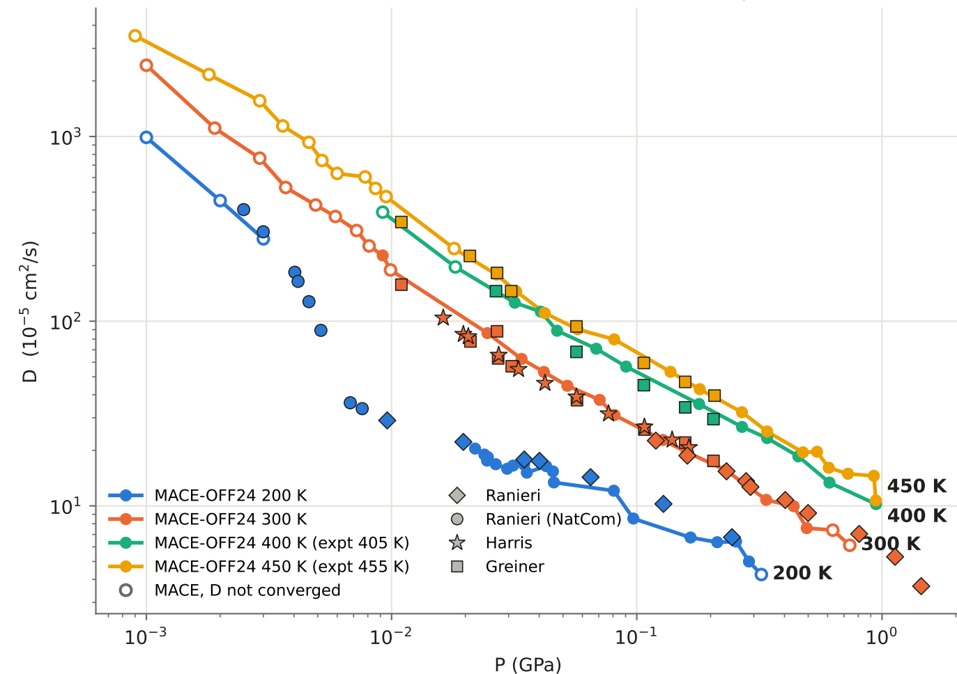
CH 4 self-diffusion: MACE-OFF24 (Yeh-Hummer corrected) vs experiment
