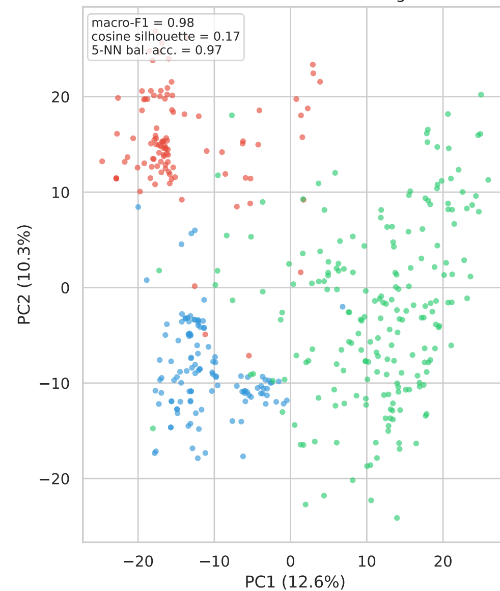
ESM2-650M test embeddings
