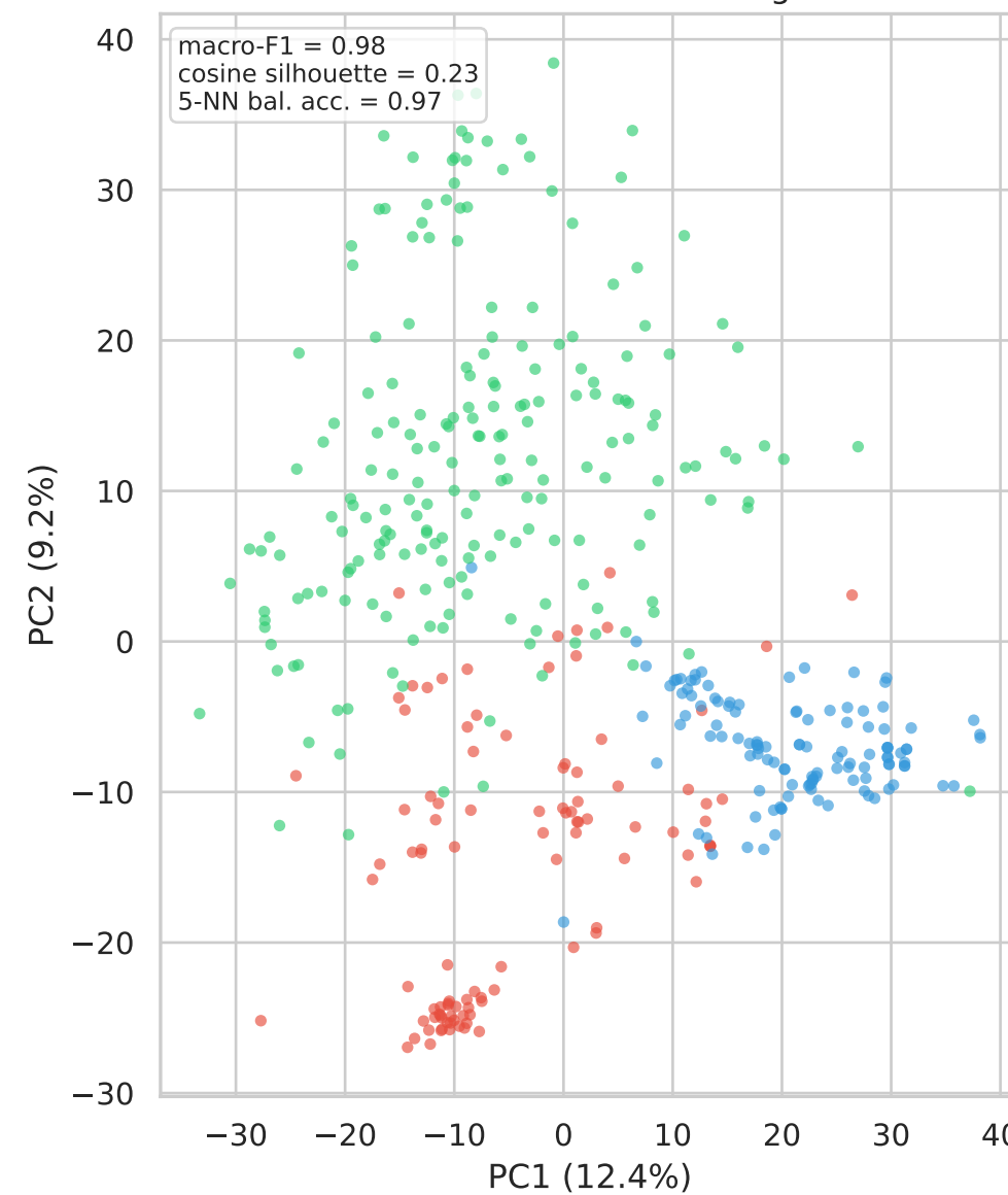
ESMC-6B test embeddings
