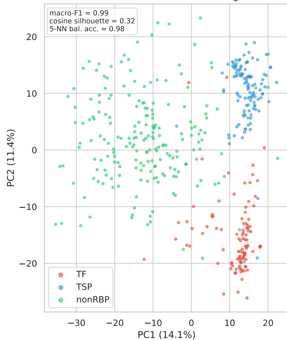
B. SaProt-650M test embeddings
