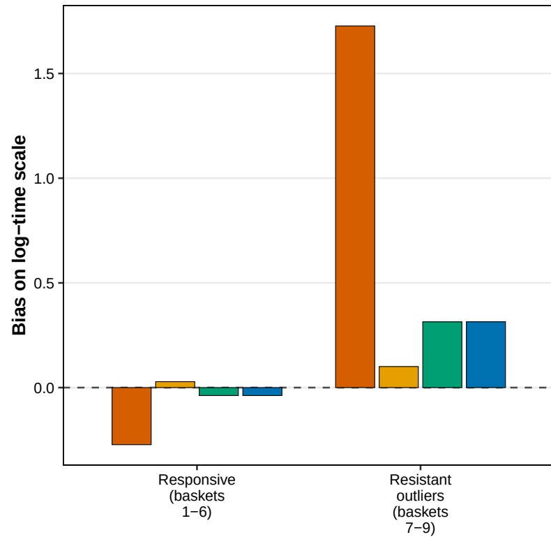
(A) Bias
