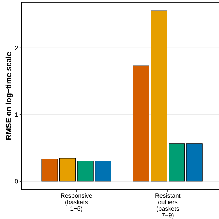
(B) RMSE
