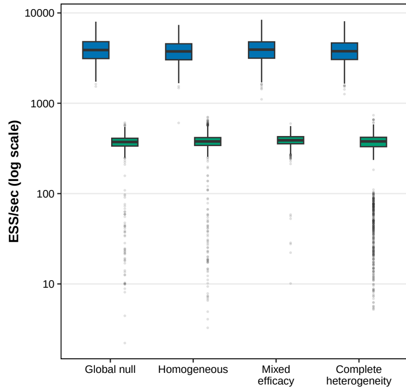
(B) Bulk ESS per second
