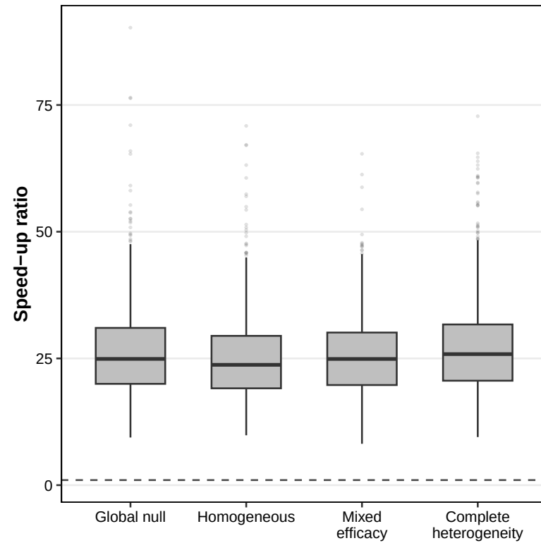
(C) Stan/Gibbs runtime ratio
