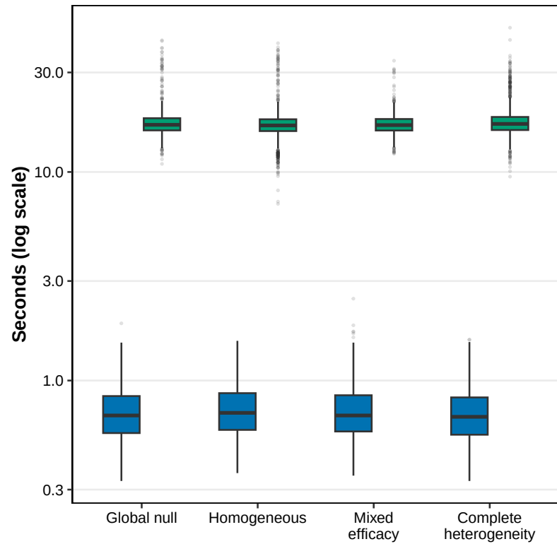
(A) Runtime per trial
