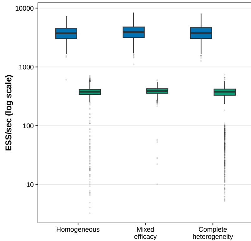
(B) Effective sample size per second
