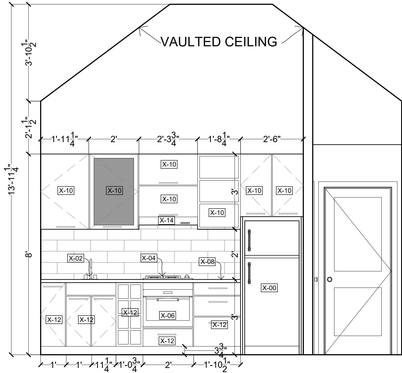
2 KITCHENETTE ELEVATION
