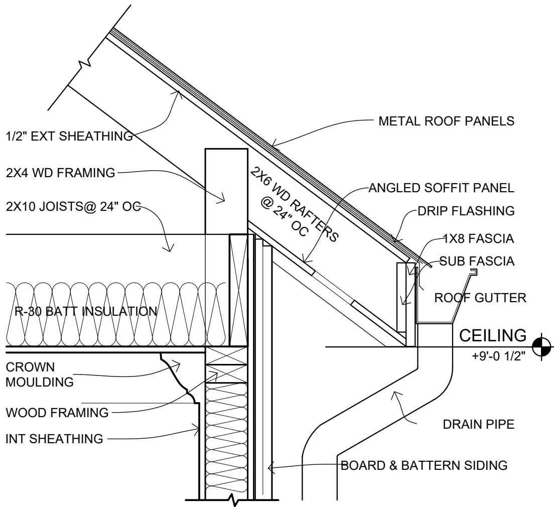
2 ROOF EAVE SECTION
