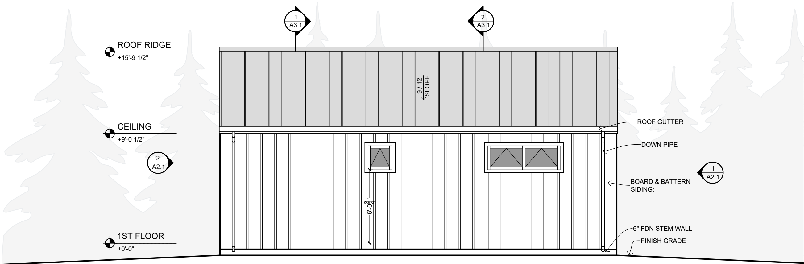
1 BACK ELEVATION (NORTH)
