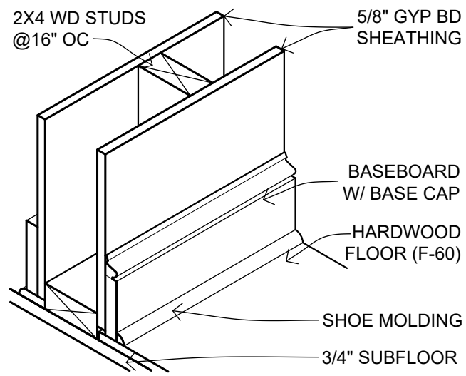
2 TYPICAL INTERIOR WALL
