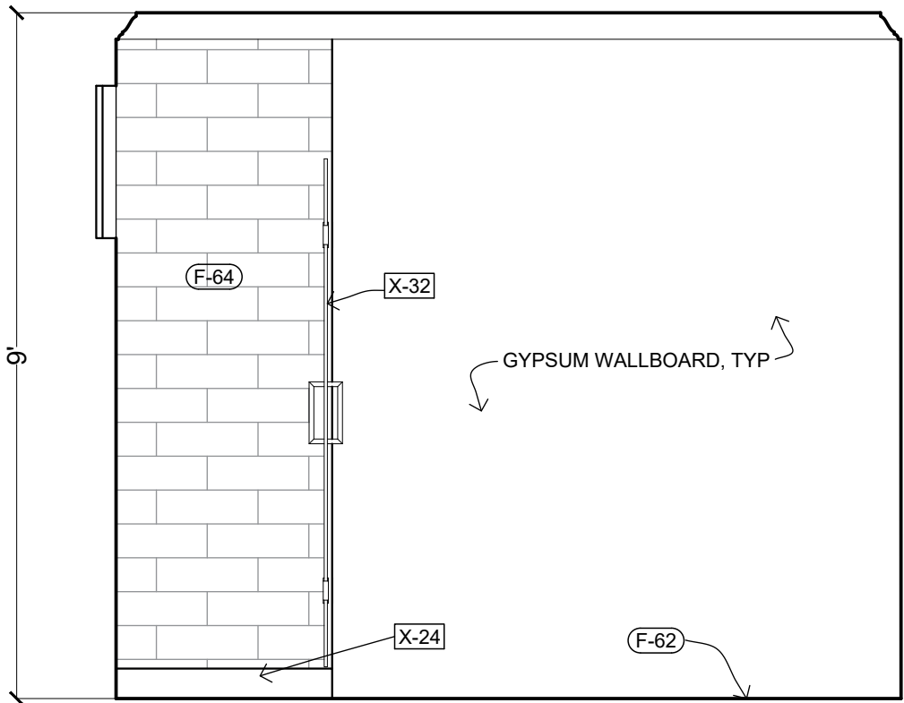
1 BATHROOM ELEVATION
