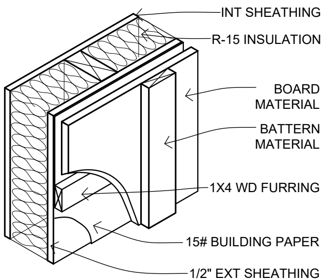
1 TYPICAL EXTERIOR WALL
