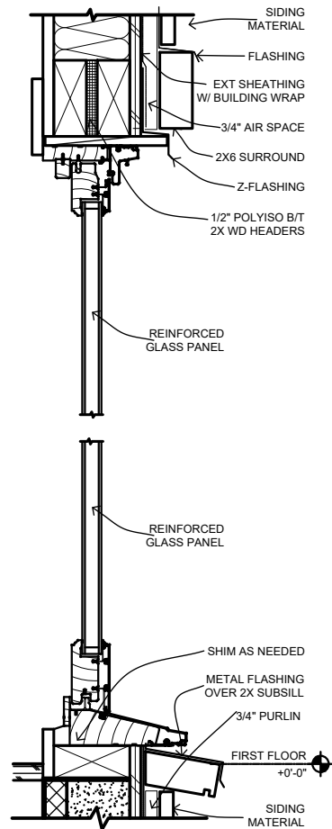
3 TYPICAL CURTAIN WALL
