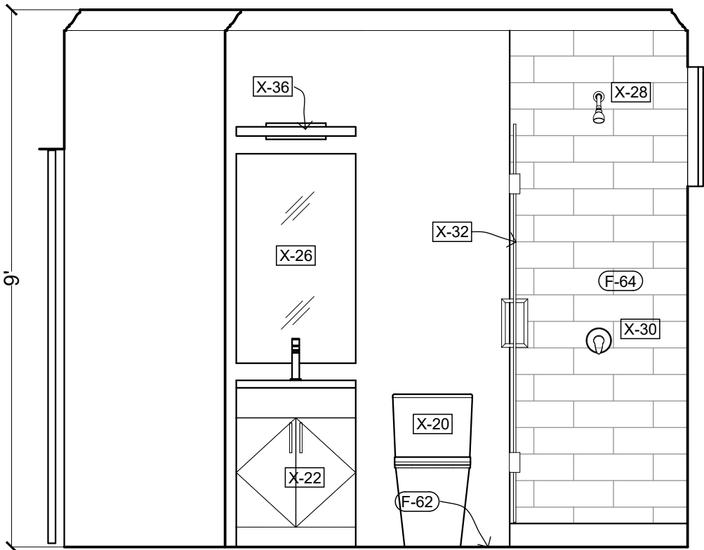
3 BATHROOM ELEVATION
