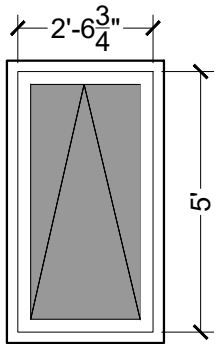
1 31" X 60"
