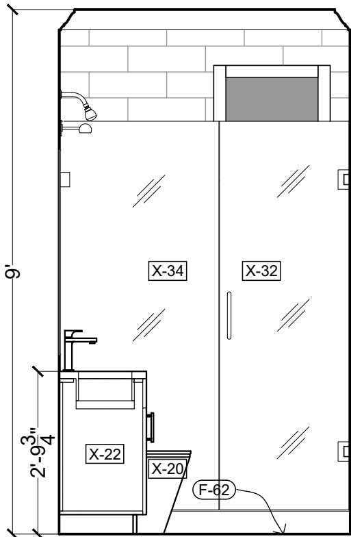
4 BATHROOM ELEVATION
