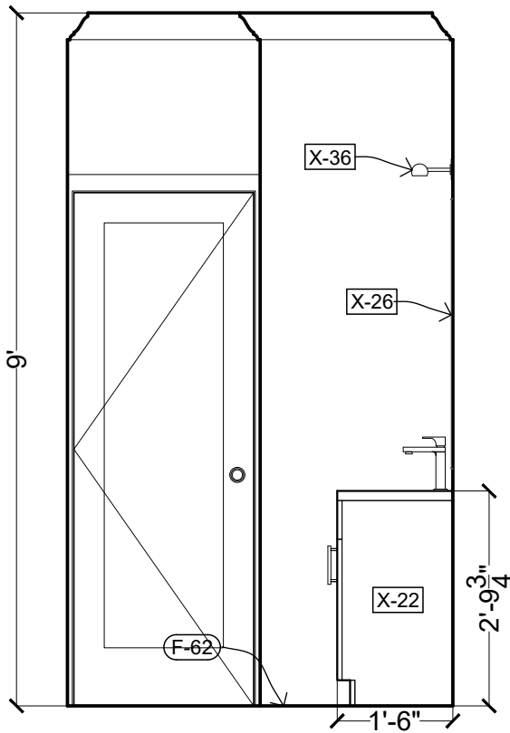
2 BATHROOM ELEVATION
