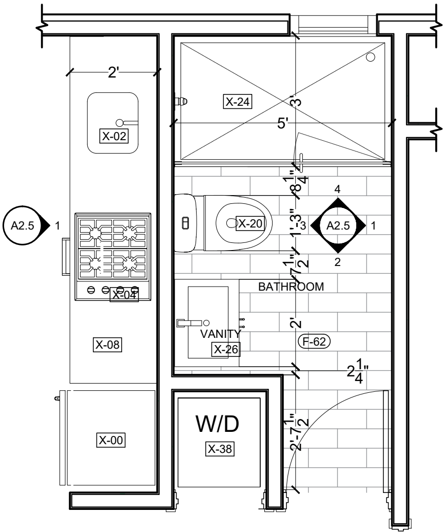
1 KITCHENETTE/ BATHROOM FLOOR PLAN DETAIL
