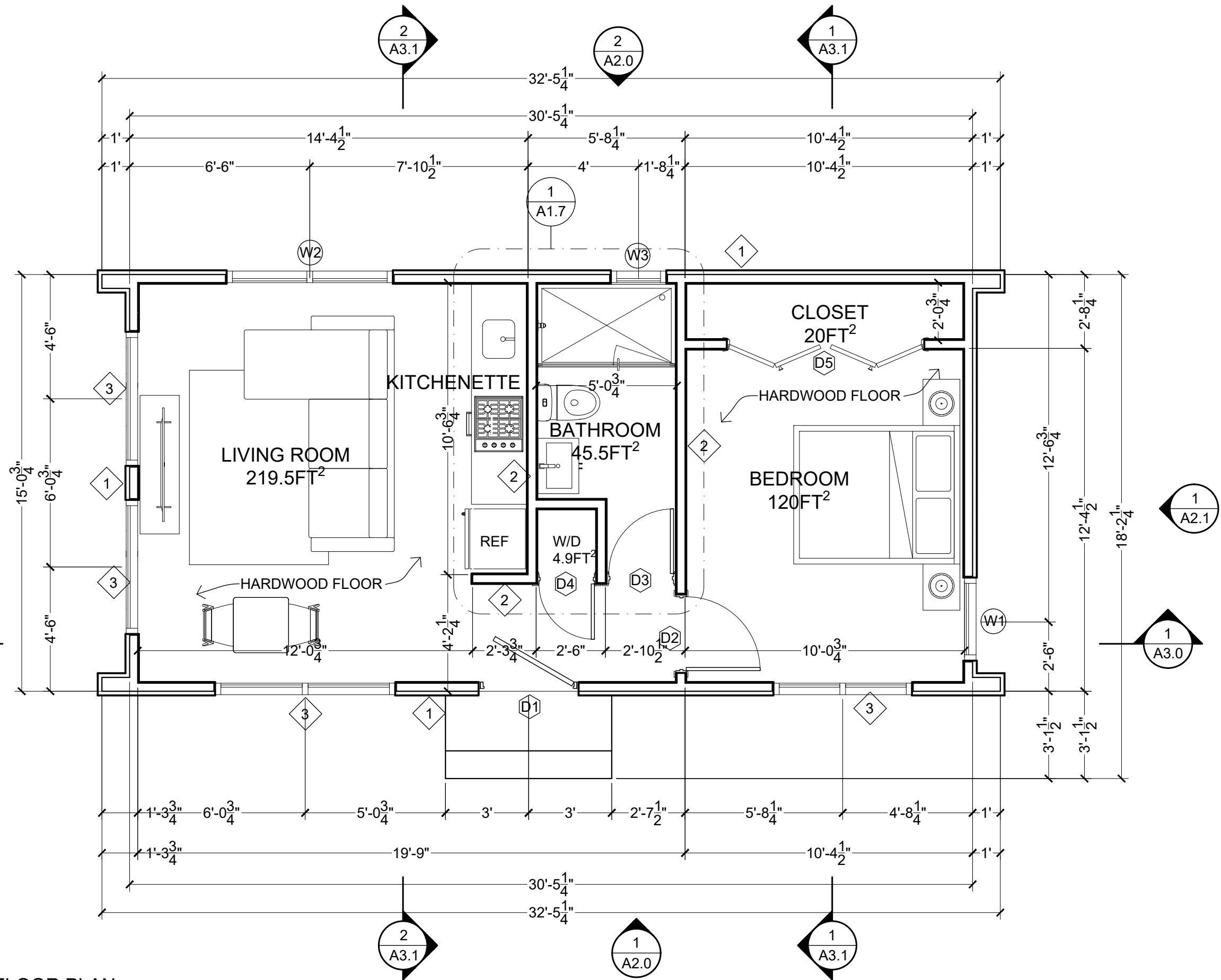
1 FIRST FLOOR PLAN
