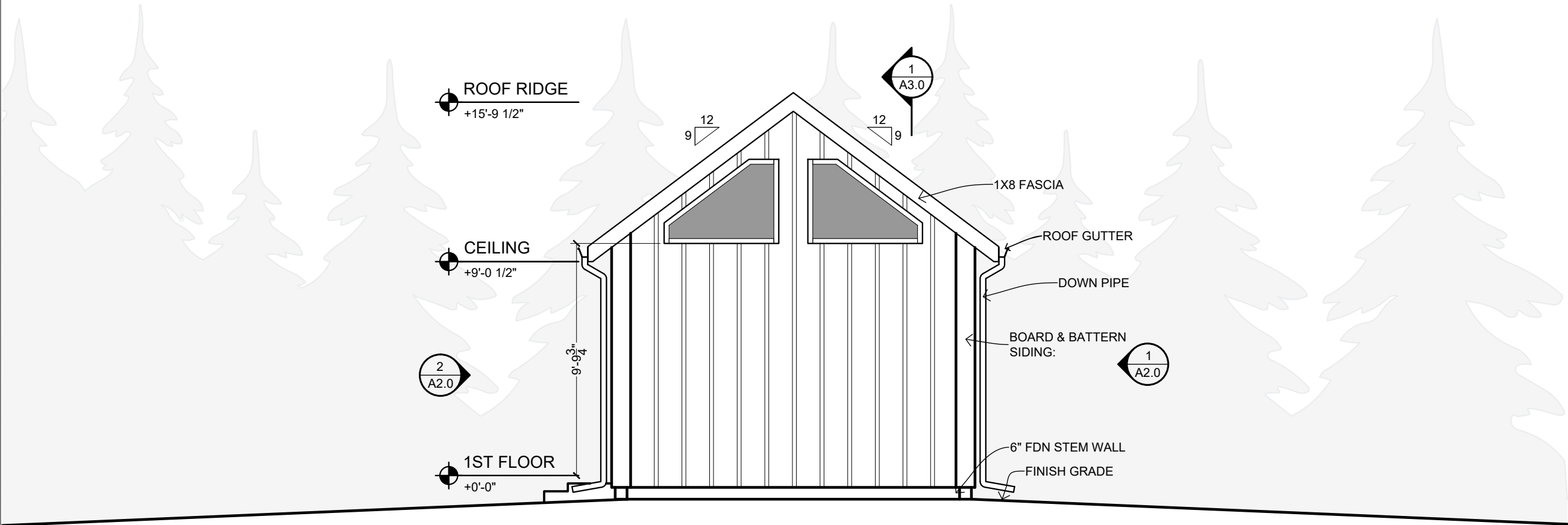
2 SIDE ELEVATION (WEST)
