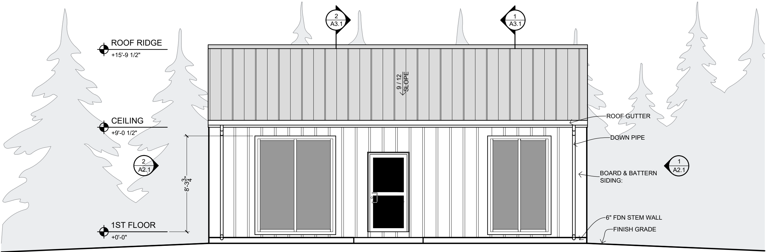
1 FRONT ELEVATION (SOUTH)
