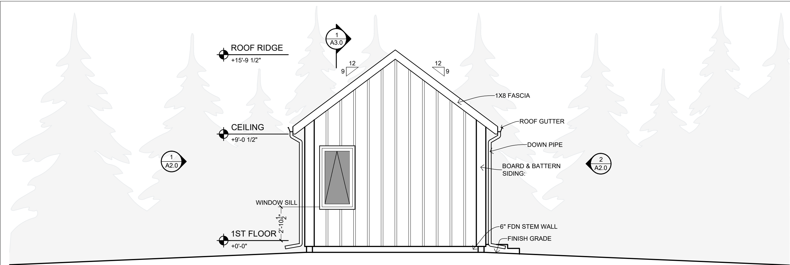
1 SIDE ELEVATION (EAST)
