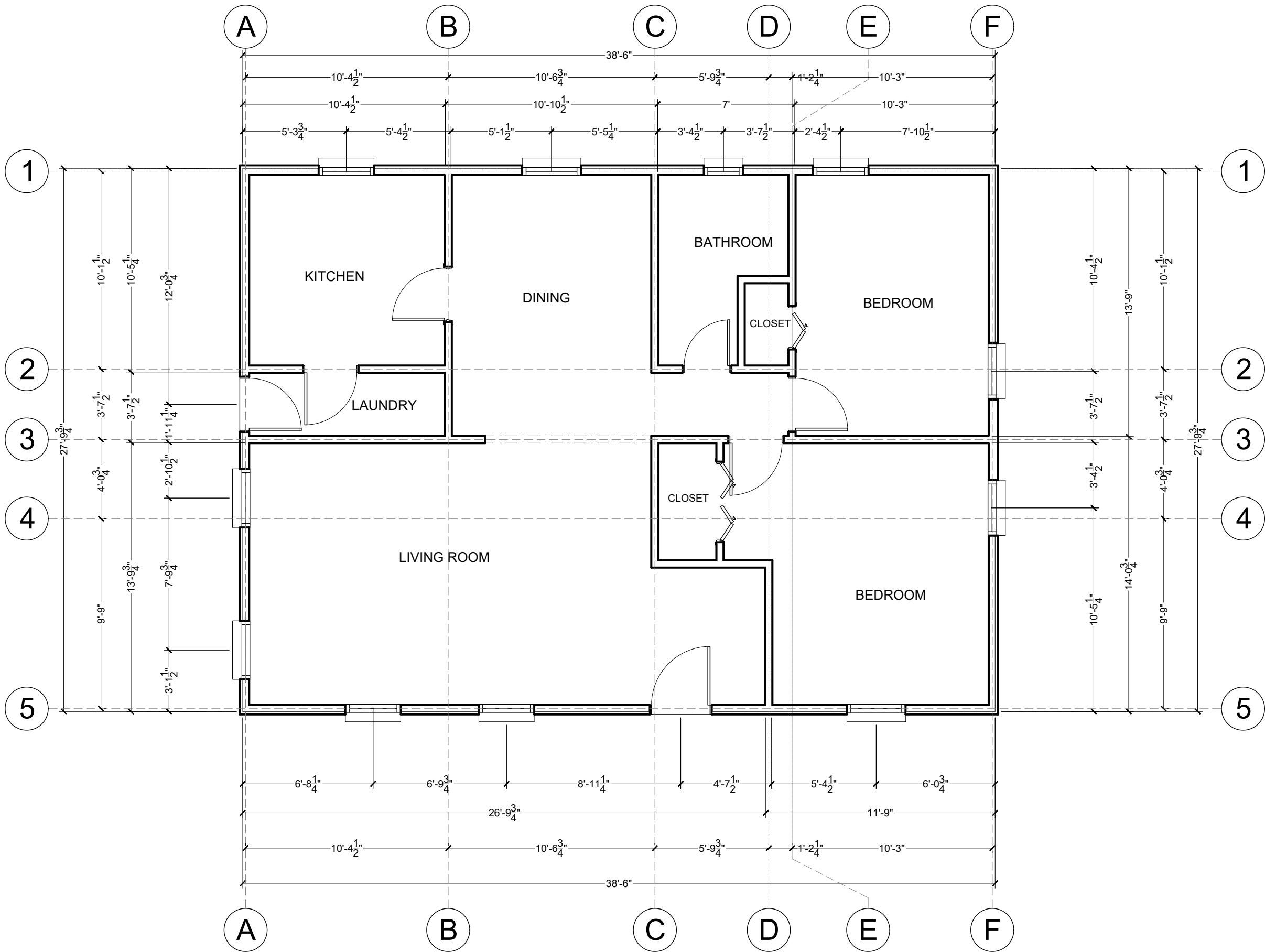
1 EXISTING FIRST FLOOR PLAN
