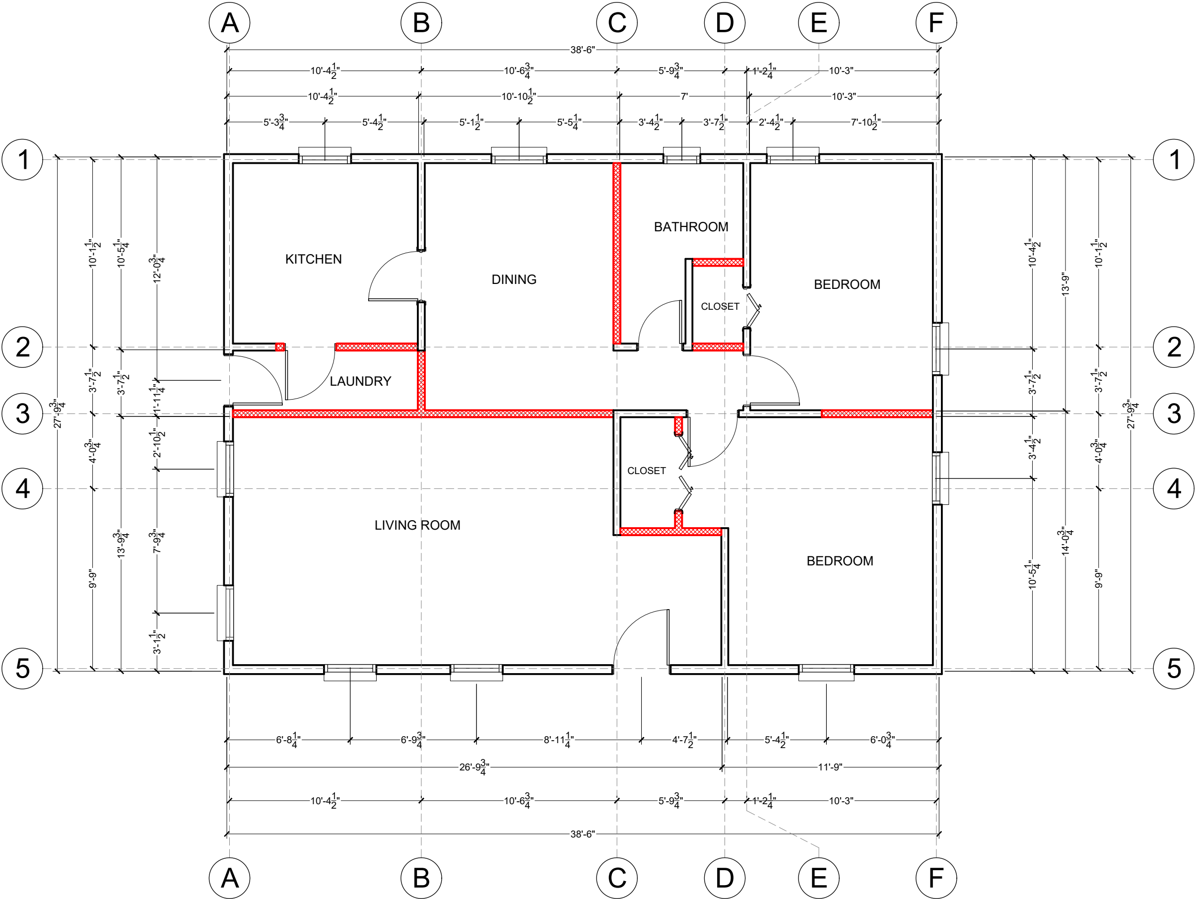
1 DEMOLITION FIRST FLOOR PLAN
