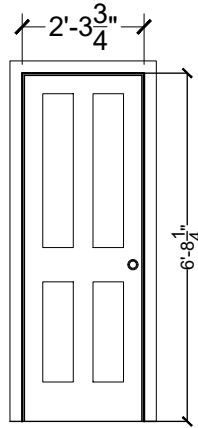
D4 BATHROOM DOOR
