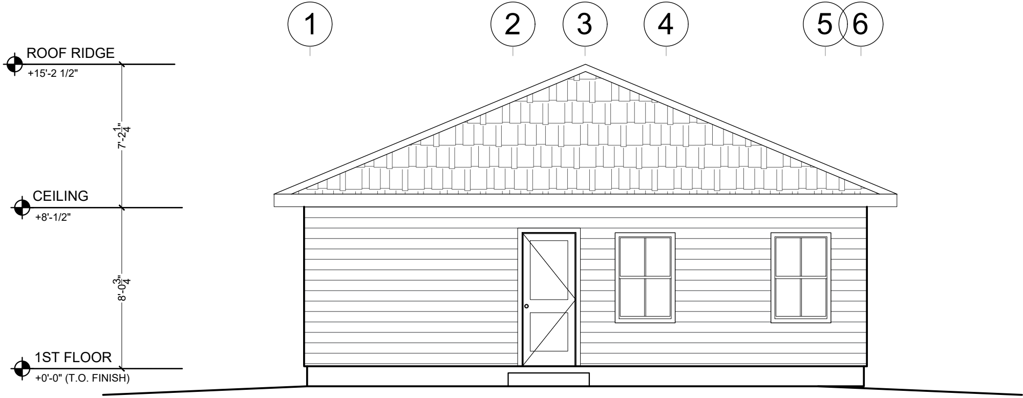
1 EXISTING SIDE ELEVATION (WEST)
