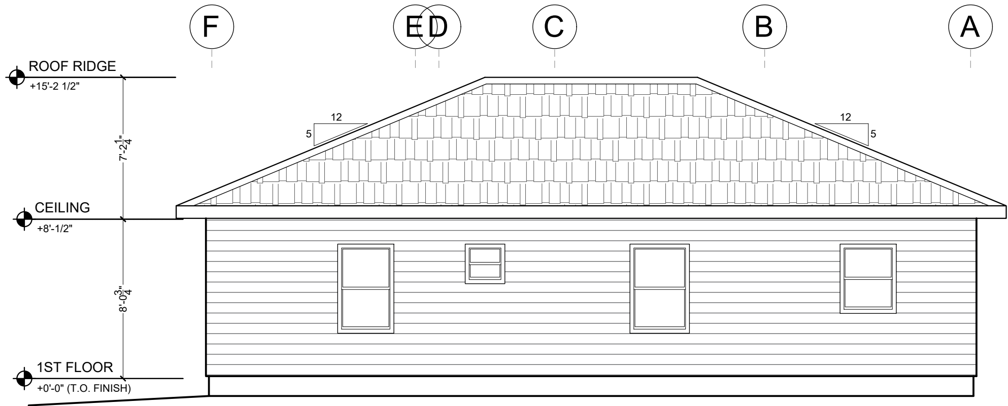
① EXISTING FRONT ELEVATION (SOUTH)
