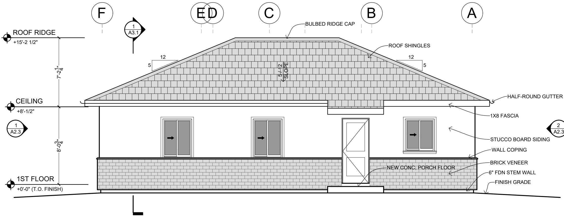
2 PROPOSED BACK ELEVATION (SOUTH)
