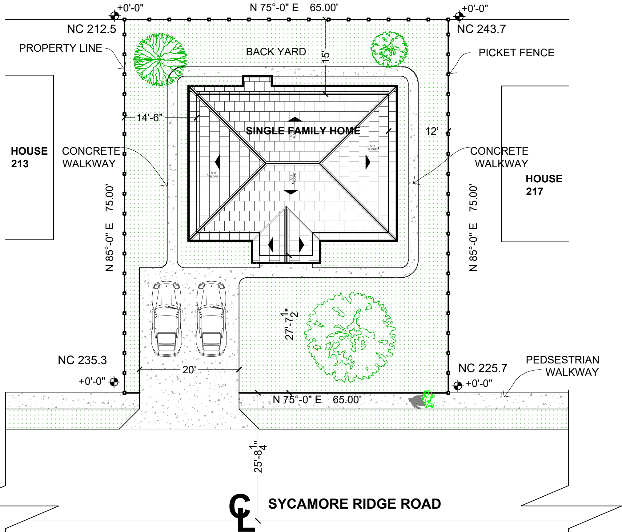
1 SITE / LANDSCAPE PLAN
