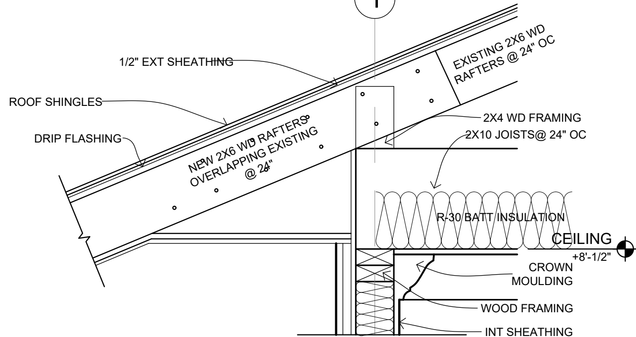
3 SHED ROOF CONNECTION TO EXISTING ROOF @ BACK PORCH
