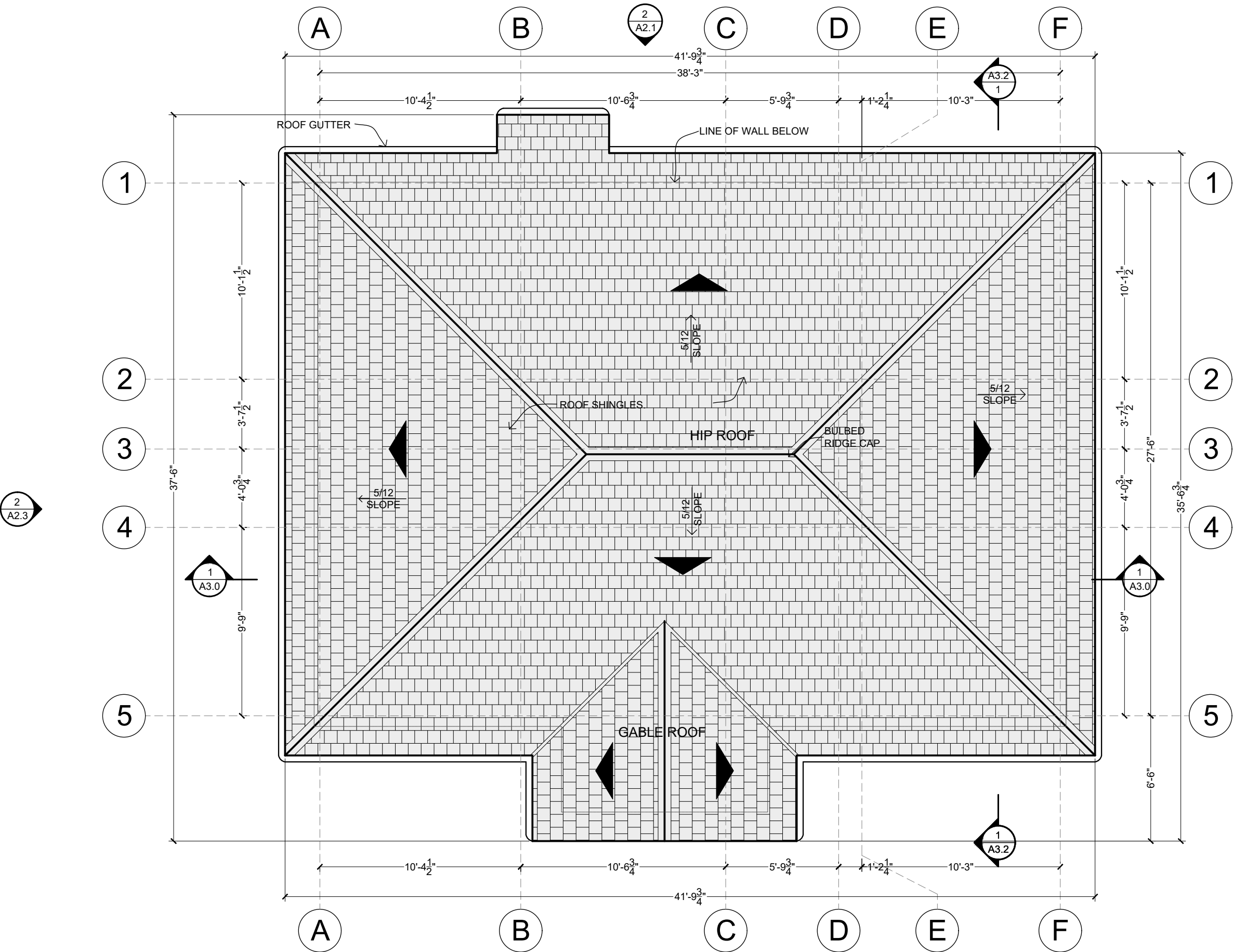
1 PROPOSED ROOF PLAN
