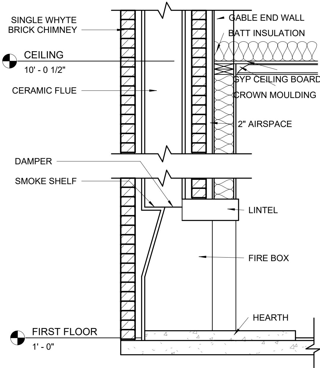
1 DETAIL SECTION THROUGH CHIMNEY 3/4" = 1'-0"
