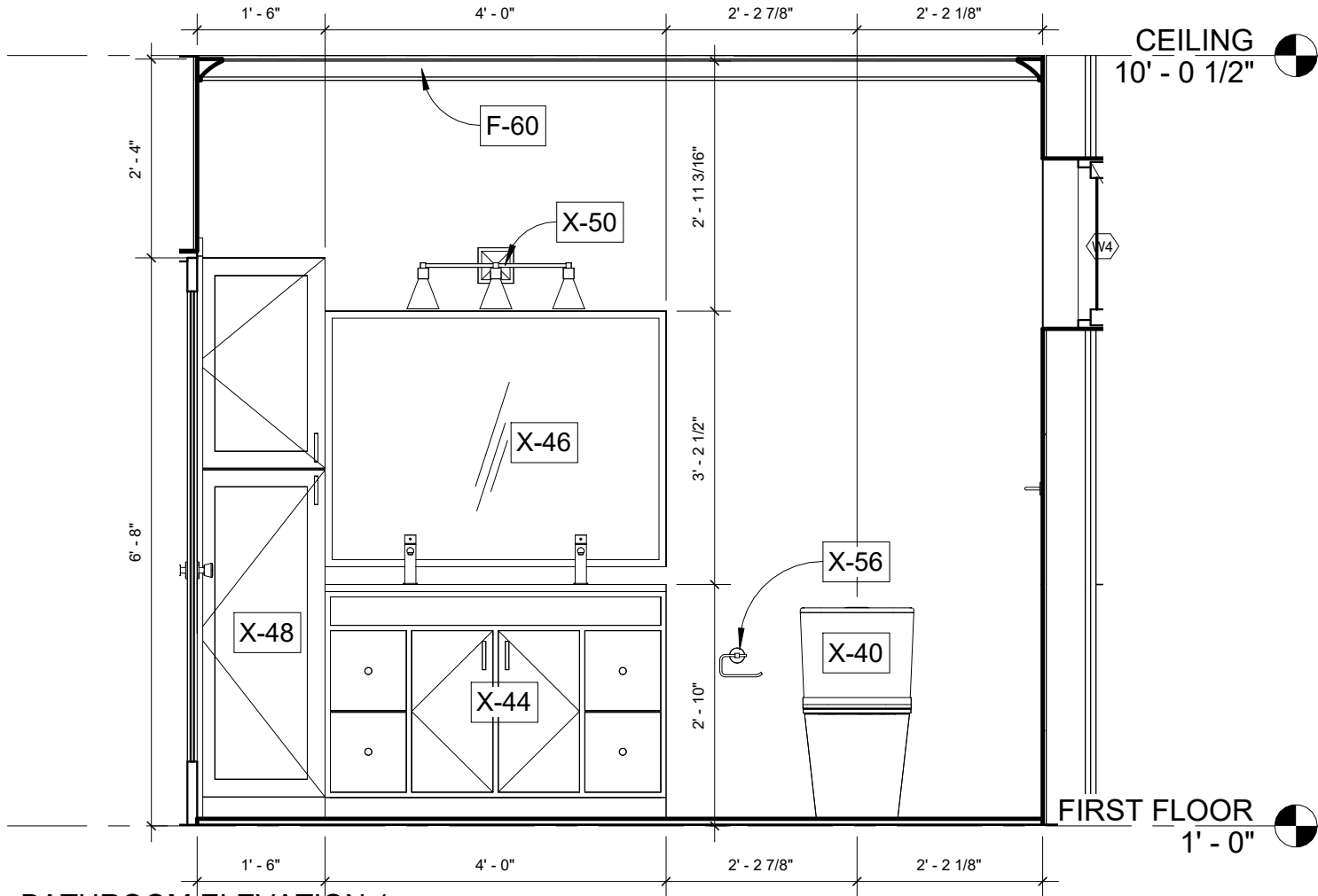
1 BATHROOM ELEVATION 1 1/2" = 1'-0"
