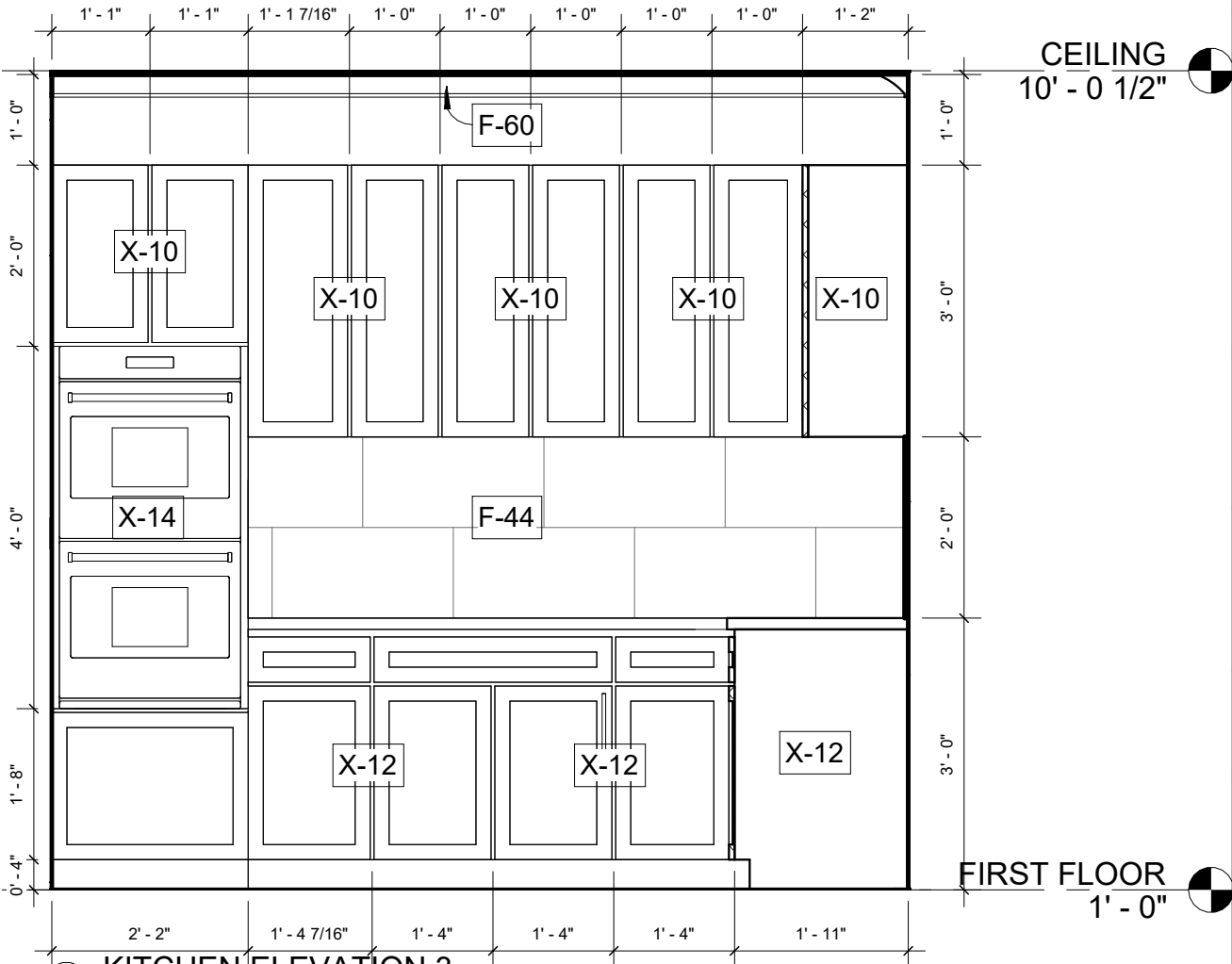
3 KITCHEN ELEVATION 3 1/2" = 1'-0"
