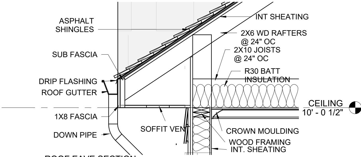
5 ROOF EAVE SECTION 3/4" = 1'-0"
