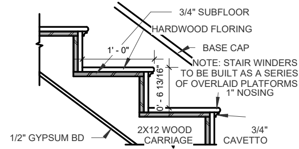
4 ATTIC STAIR SECTION DETAIL 3/4" = 1'-0"
