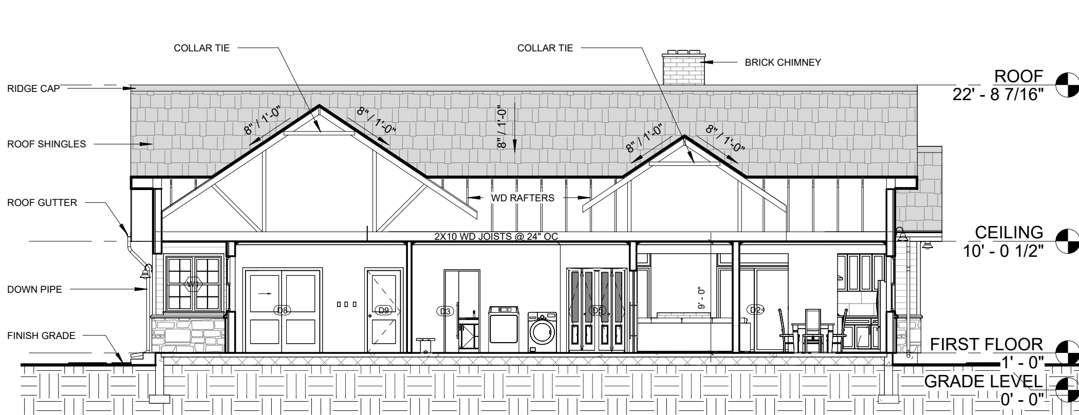
2 Section 2 1/8" = 1'-0"
