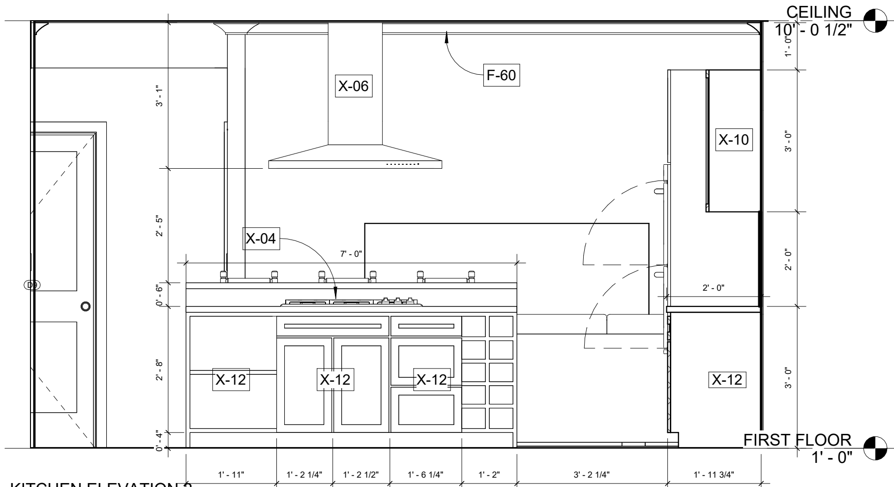
2 KITCHEN ELEVATION 2 1/2" = 1'-0"
