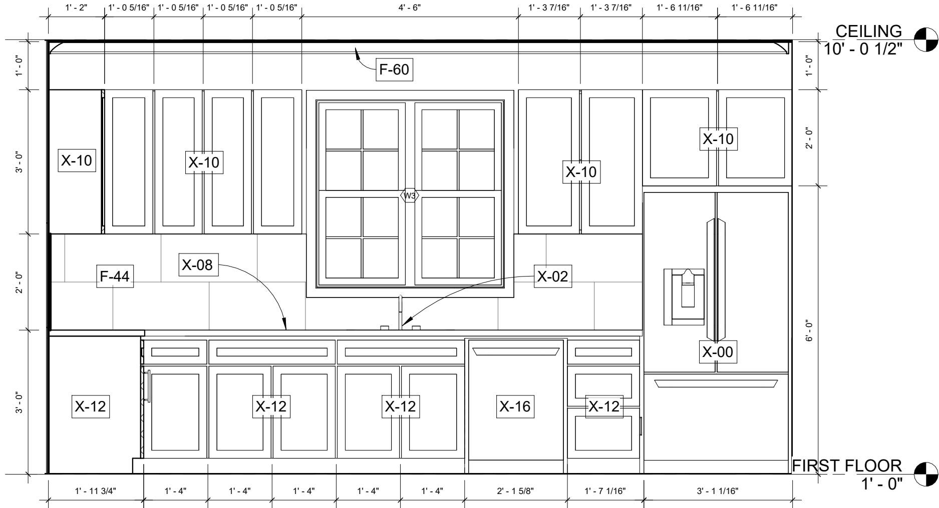
1 KITCHEN ELEVATION 1 1/2" = 1'-0"
