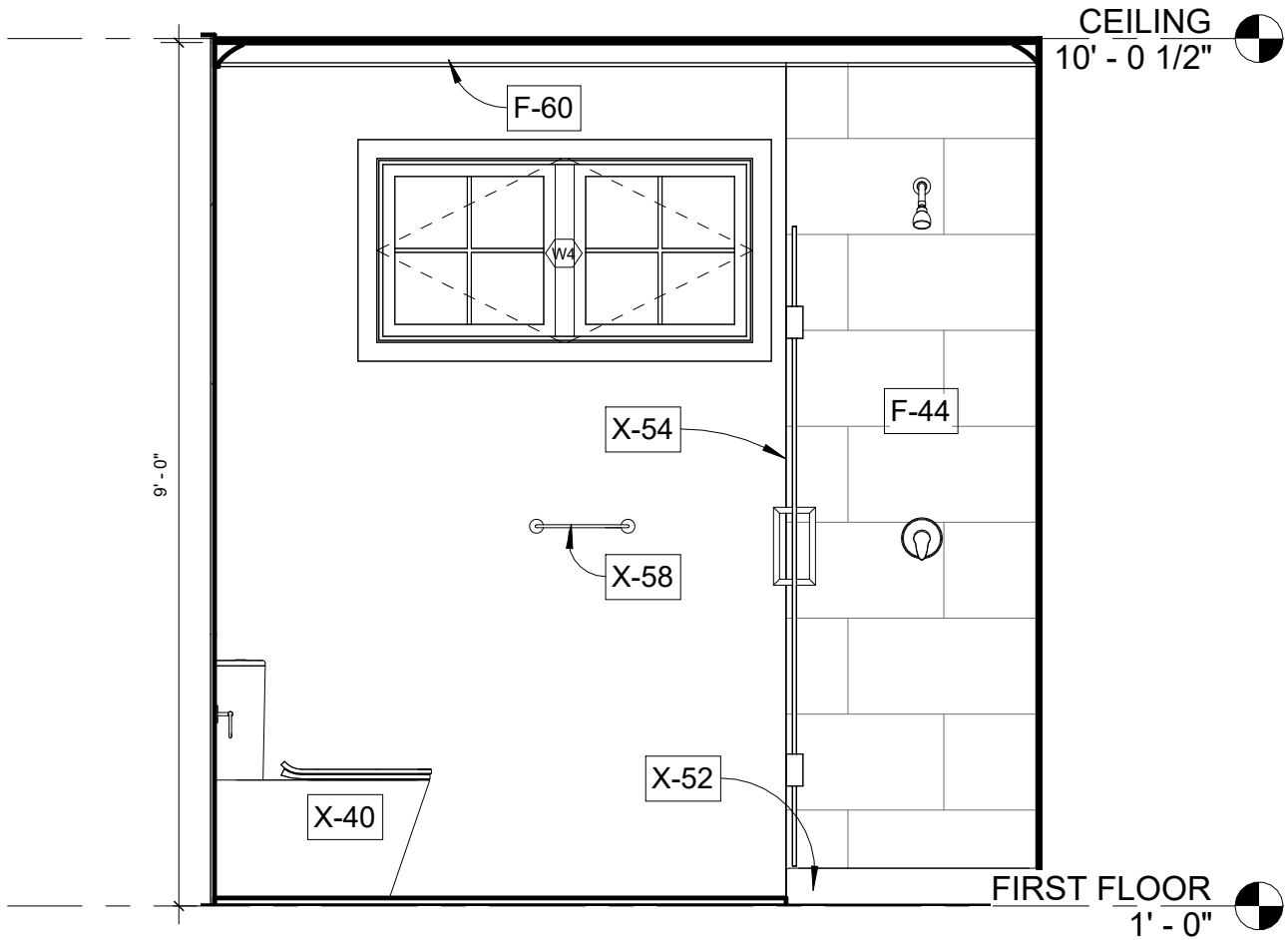
2 BATHROOM ELEVATION 2 1/2" = 1'-0"
