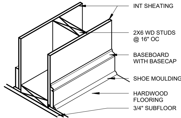
7 TYP INT WALL 1" = 1'-0"
