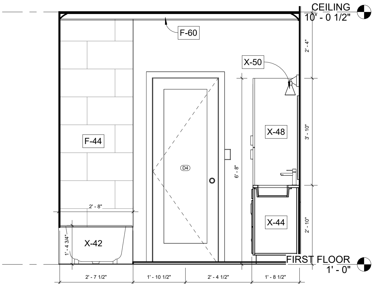
4 BATHROOM ELEVATION 4 1/2" = 1'-0"
