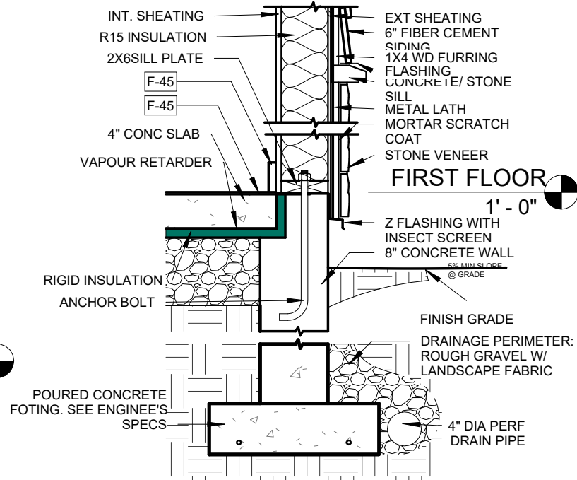
3 FOUNDATION DETAIL 3/4" = 1'-0"
