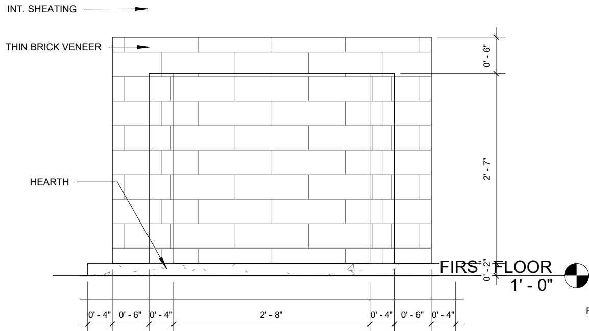
2 CHIMNEY ELEVATION 3/4" = 1'-0"
