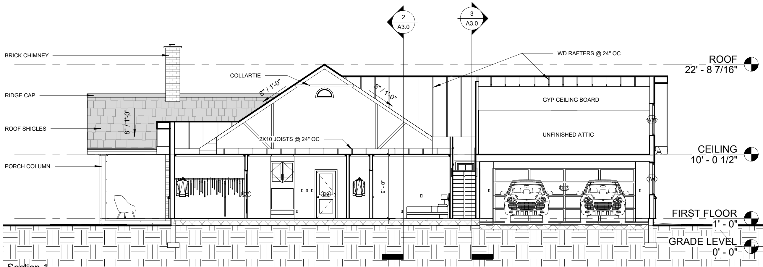
1 Section 1 1/8" = 1'-0"
