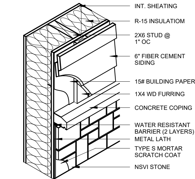
6 TYP EXT WALL 1" = 1'-0"
