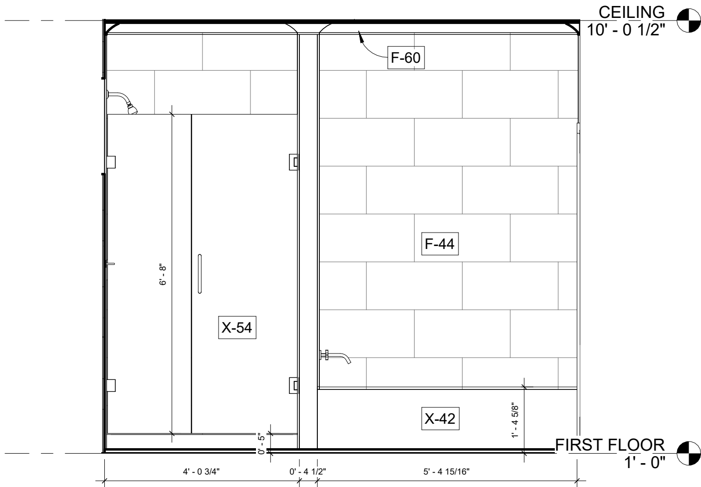
3 BATHROOM ELEVATION 3 1/2" = 1'-0"
