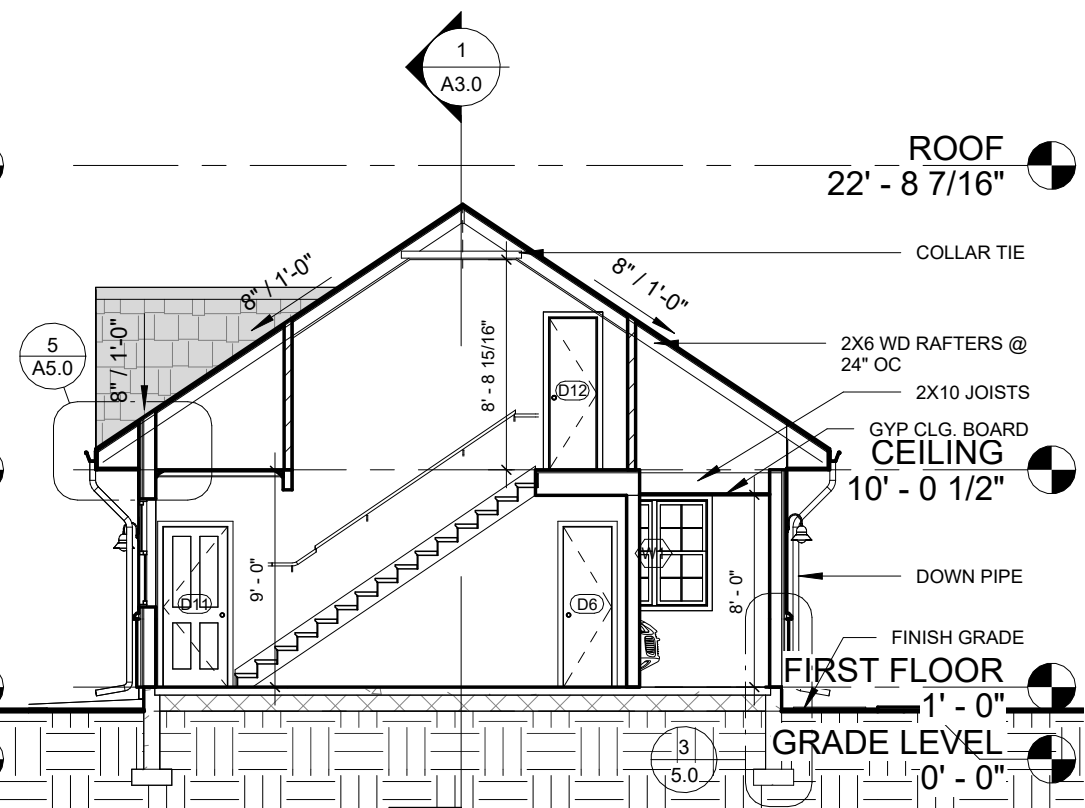
3 Section 3 1/8" = 1'-0"
