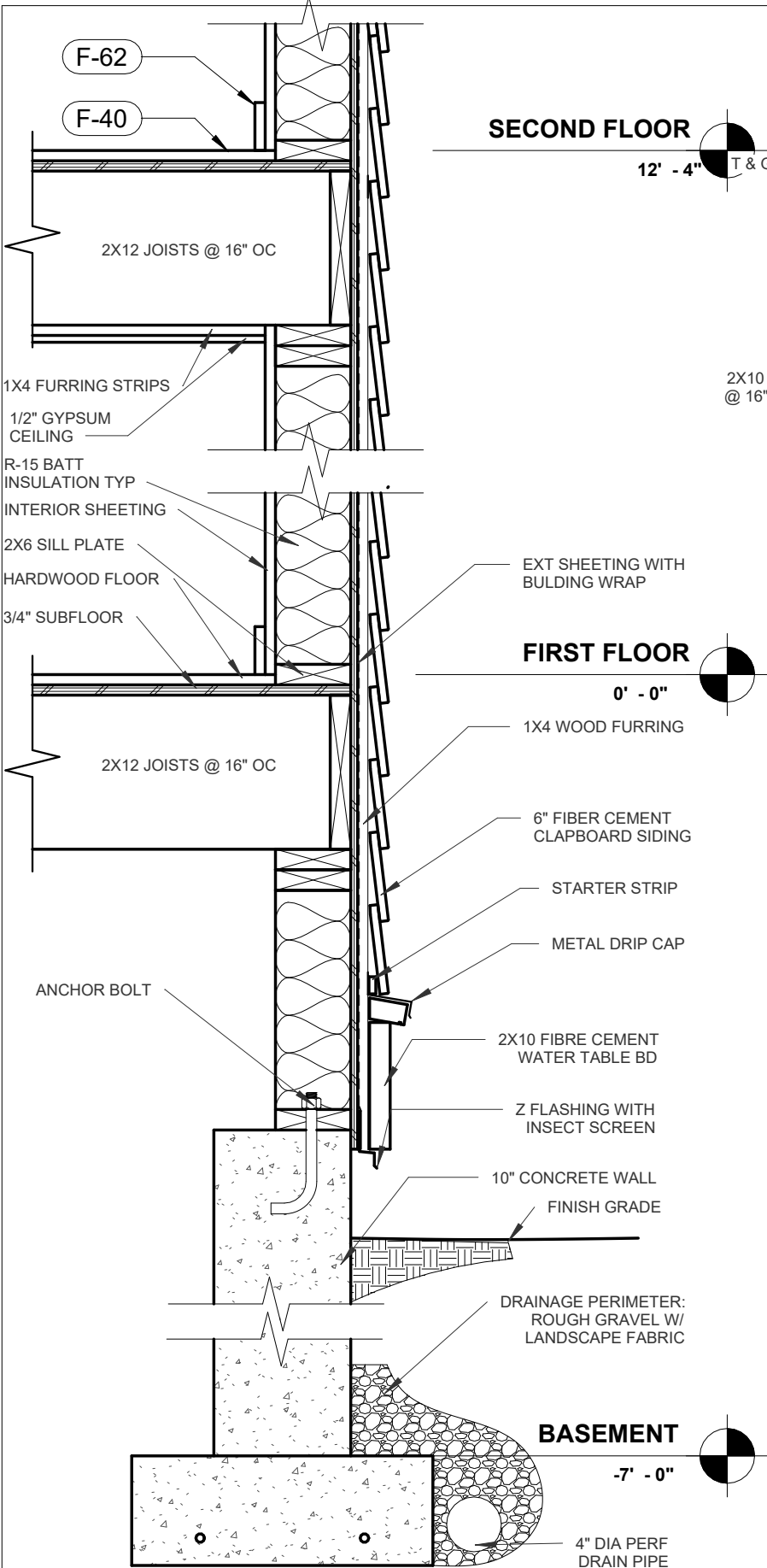
1 WALL SECTION DETAILS 1" = 1'-0"
