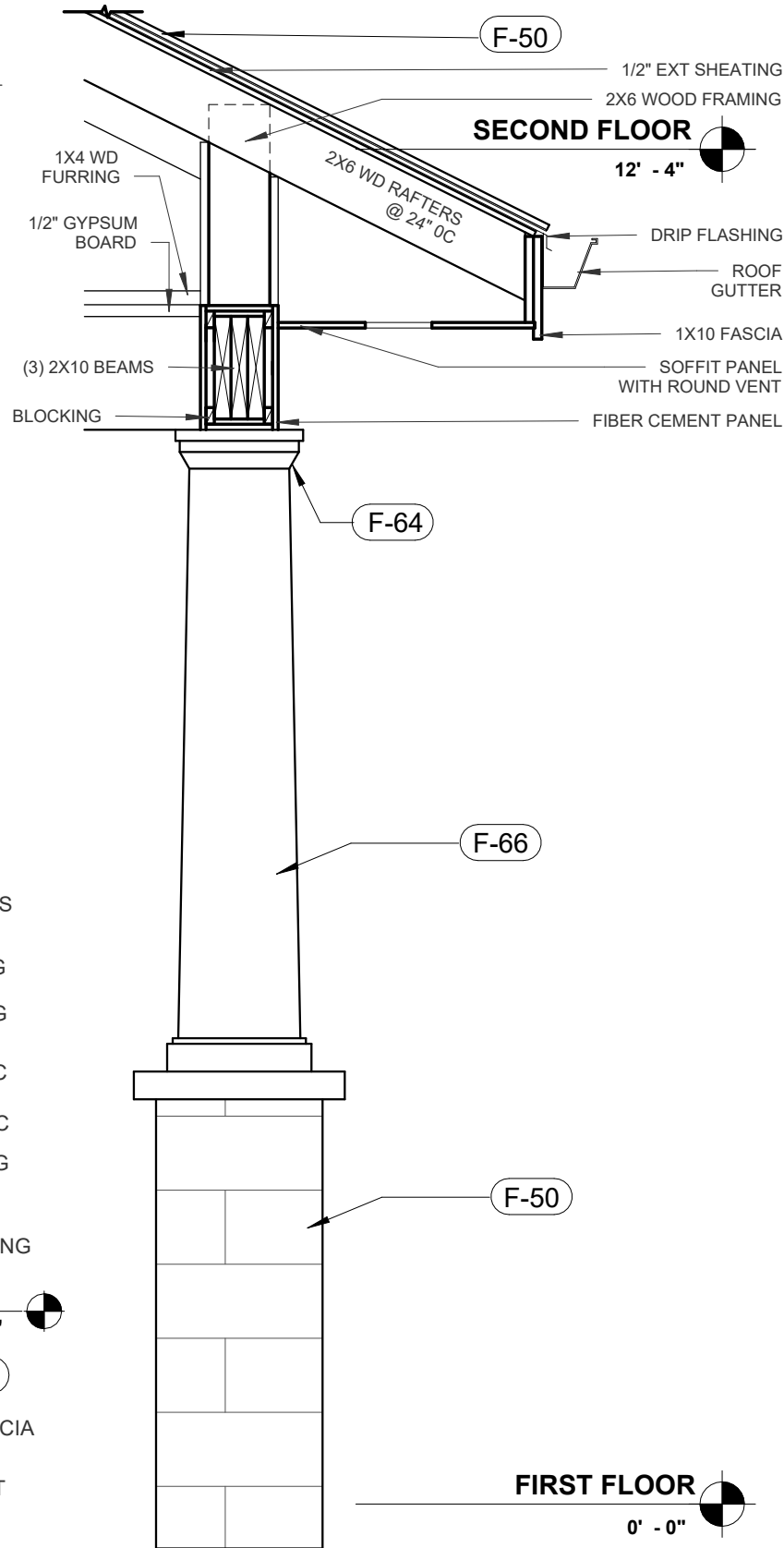
4 FRONT PORCH COLUMN 3/4" = 1'-0"
