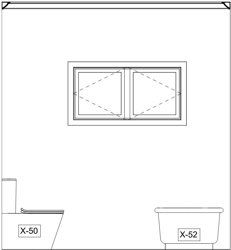
2 BATHROOM ELEVATION 2 1/2" = 1'-0"
