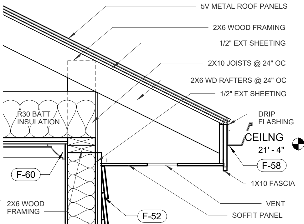
2 ROOF EAVE DETAIL 1" = 1'-0"
