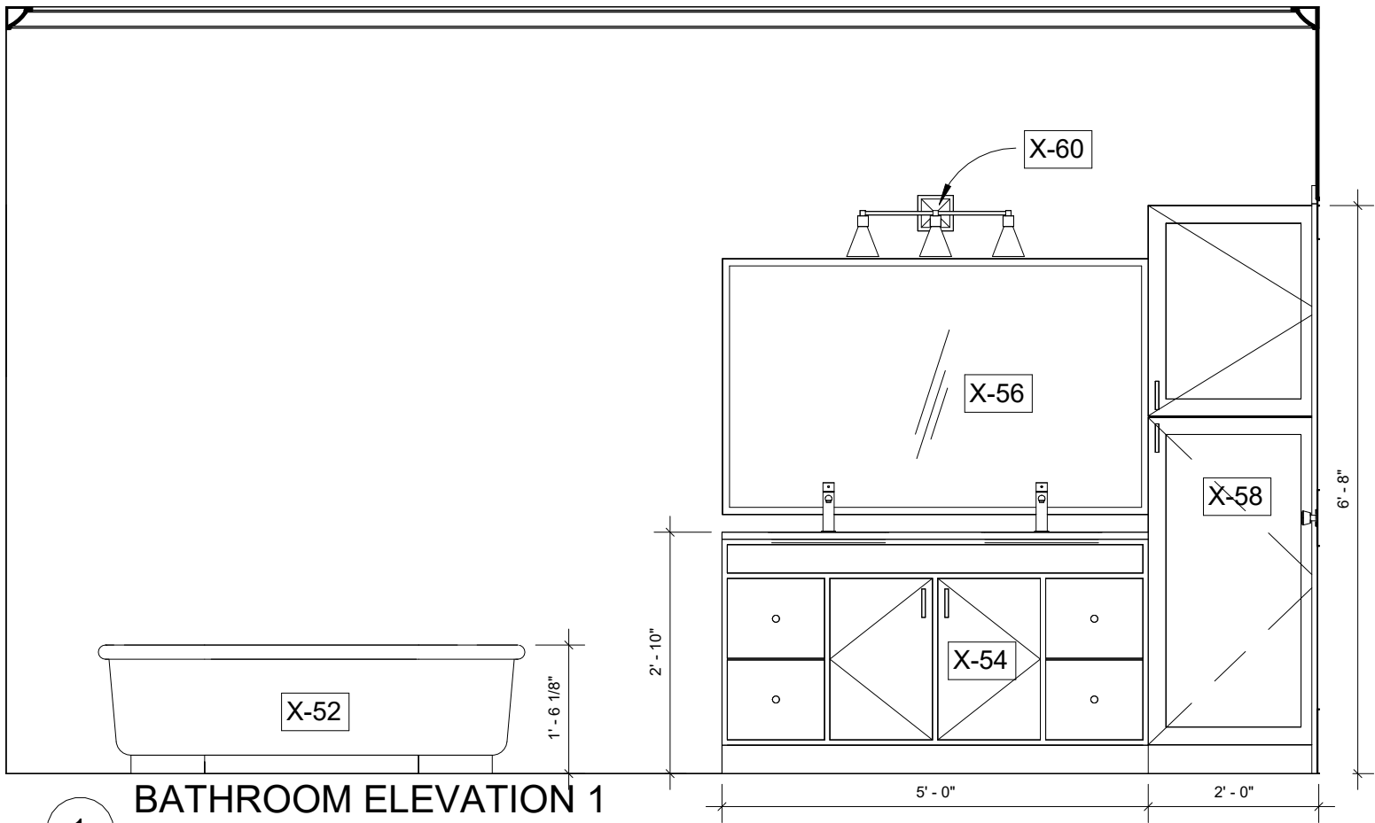
1 BATHROOM ELEVATION 1 1/2" = 1'-0"
