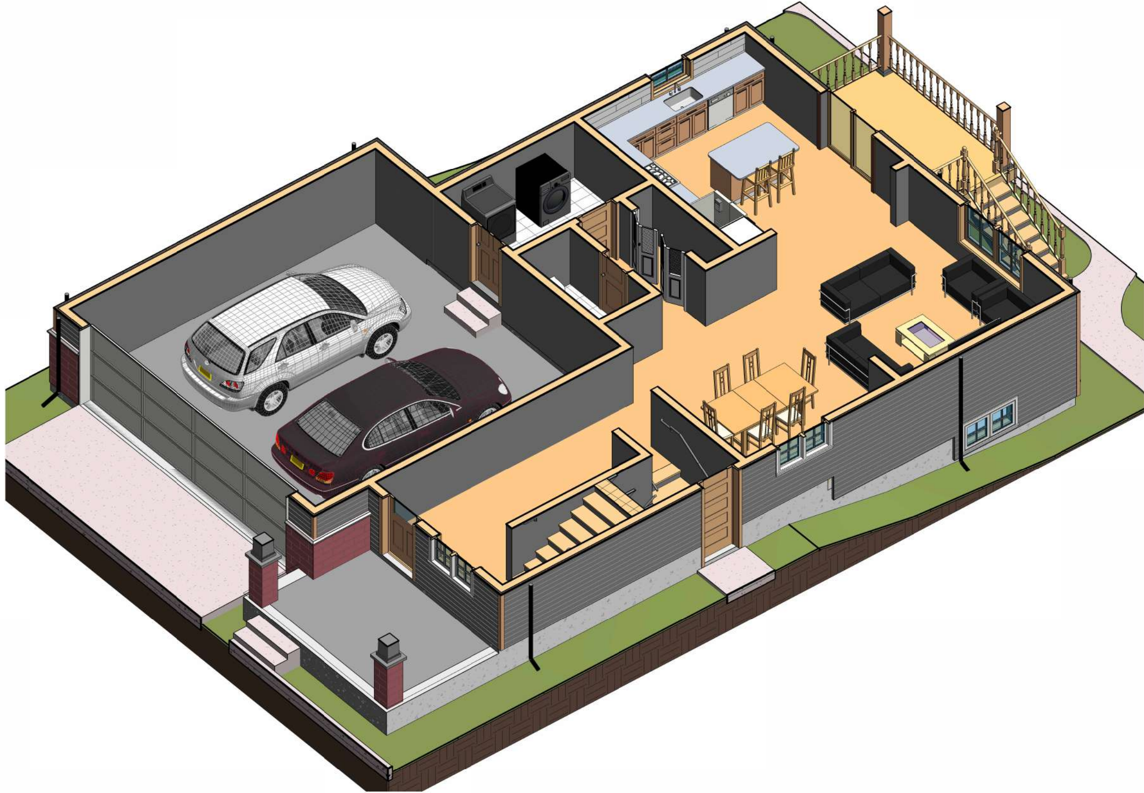
AXONOMETRIC VIEW (1ST FLOOR)
