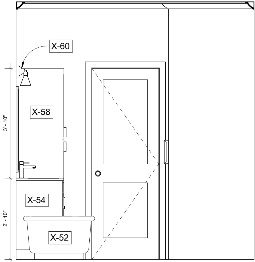
4 BATHROOM ELEVATION 4 1/2" = 1'-0"
