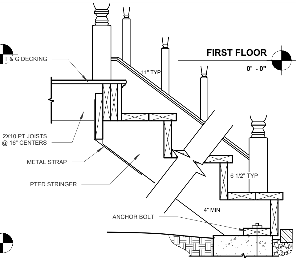
3 DECK STAIRS DETAILS 1" = 1'-0"
