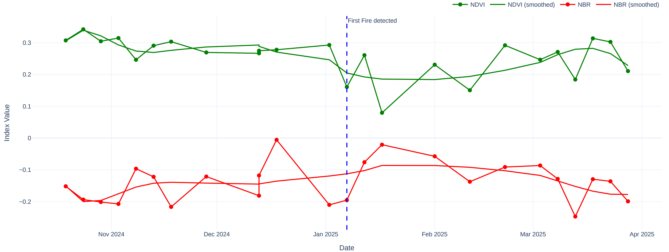
NDVI and NBR TimeSeries
