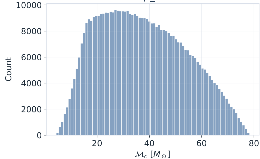
chirp_mass
