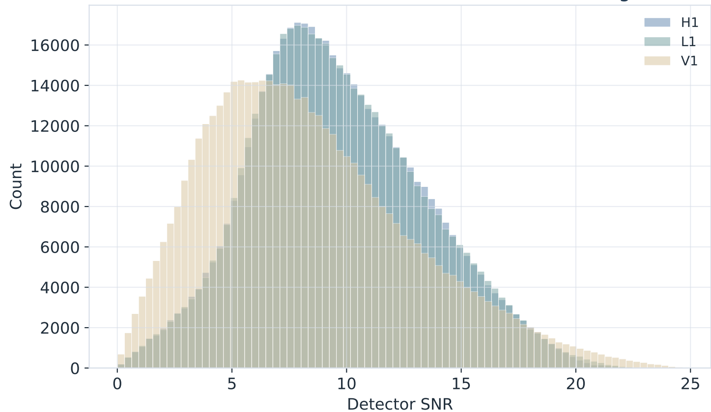
Detector-level SNR distributions after rescaling
