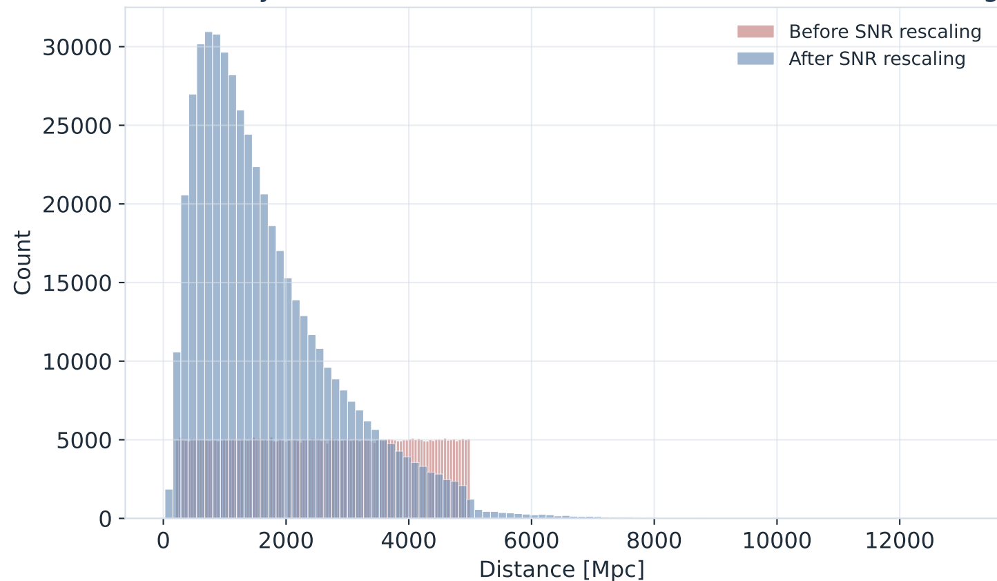
Luminosity-distance distribution before and after SNR rescaling
