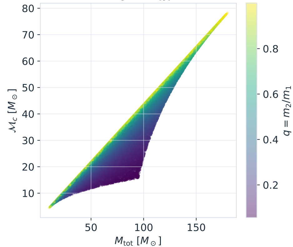
\mathcal{M}_c vs M_{\text{tot}}
