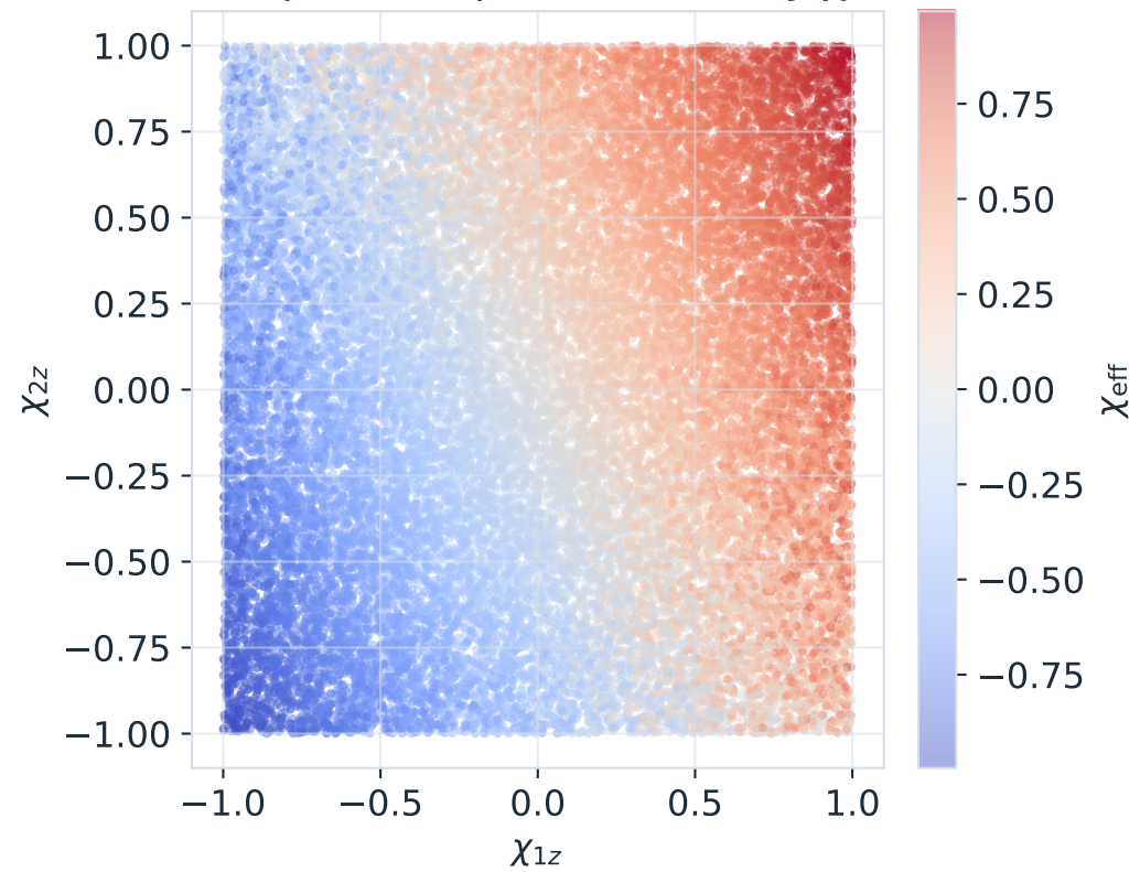
Component spins colored by \chi_{\text{eff}}
