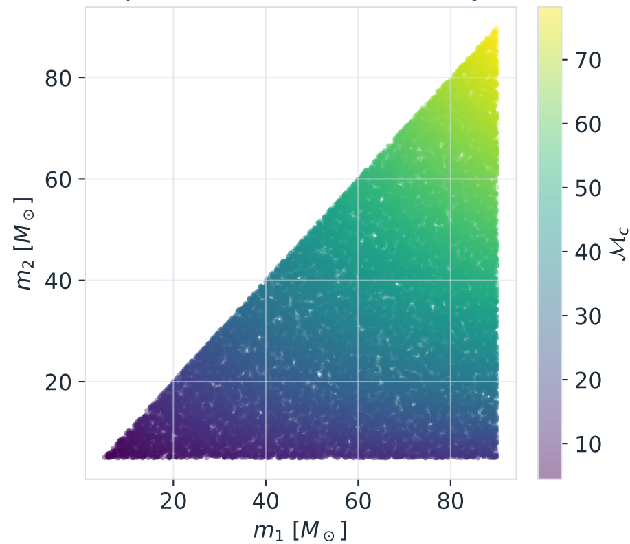
Component masses colored by \mathcal{M}_c
