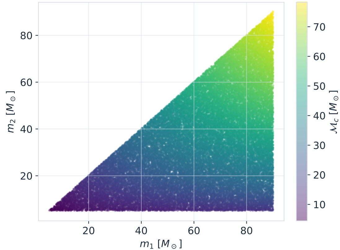
Component masses \rightarrow chirp mass
