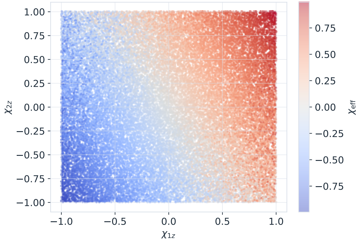
Component spins \rightarrow \chi_{\text{eff}}
