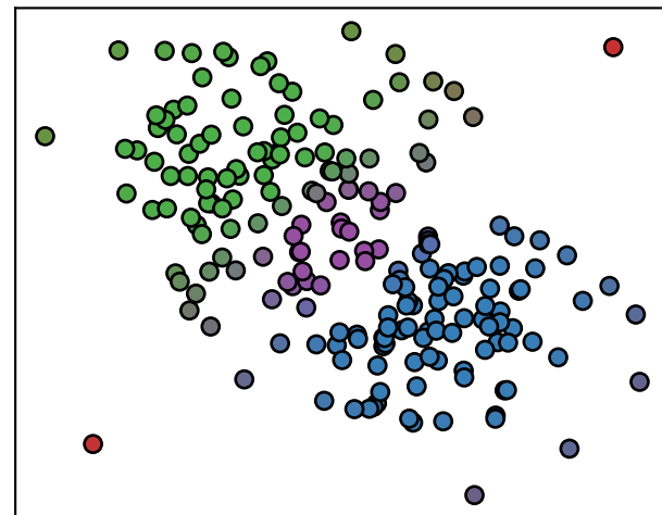
Evidential Clustering ( \alpha = 1 , \beta = 1.4 , \delta = 3 )
