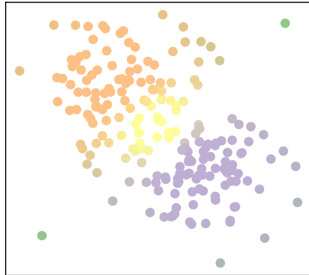
Evidential Clustering
