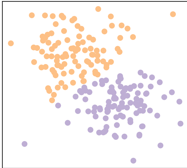
Hard Clustering
