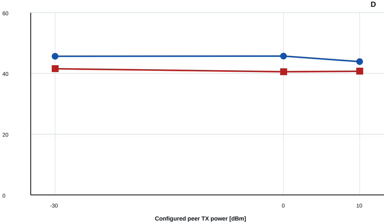
RX power above standby
