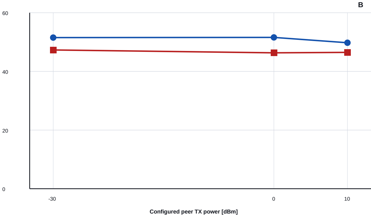
Total RX power
