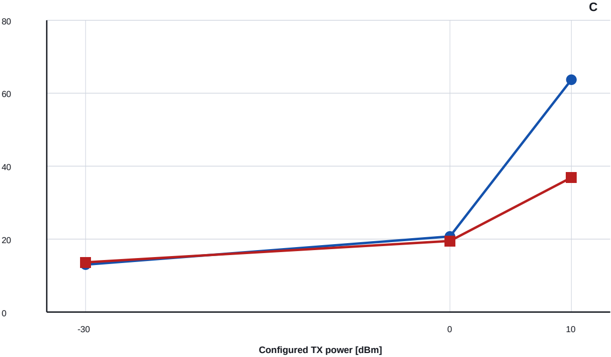
TX power above standby
