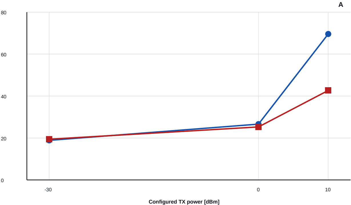
Total TX power
