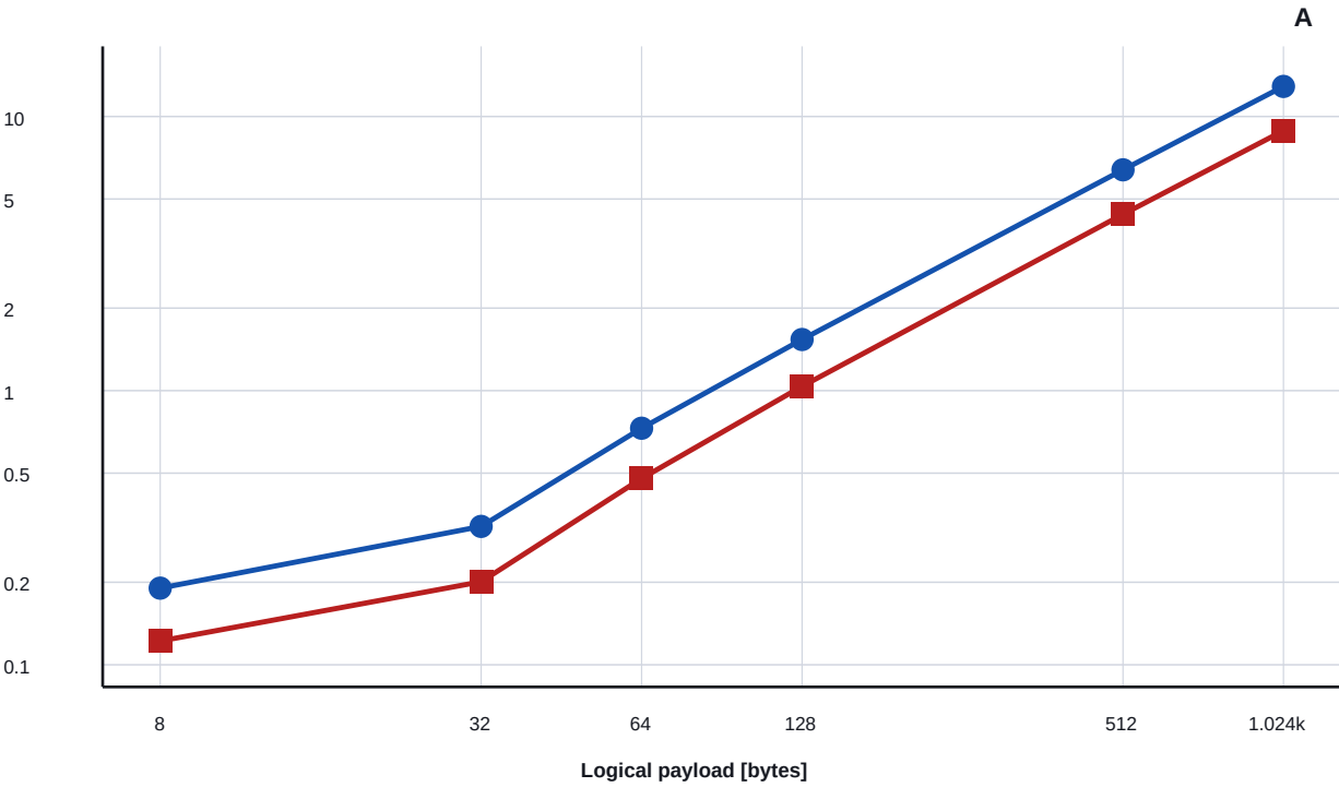
TX energy versus payload
