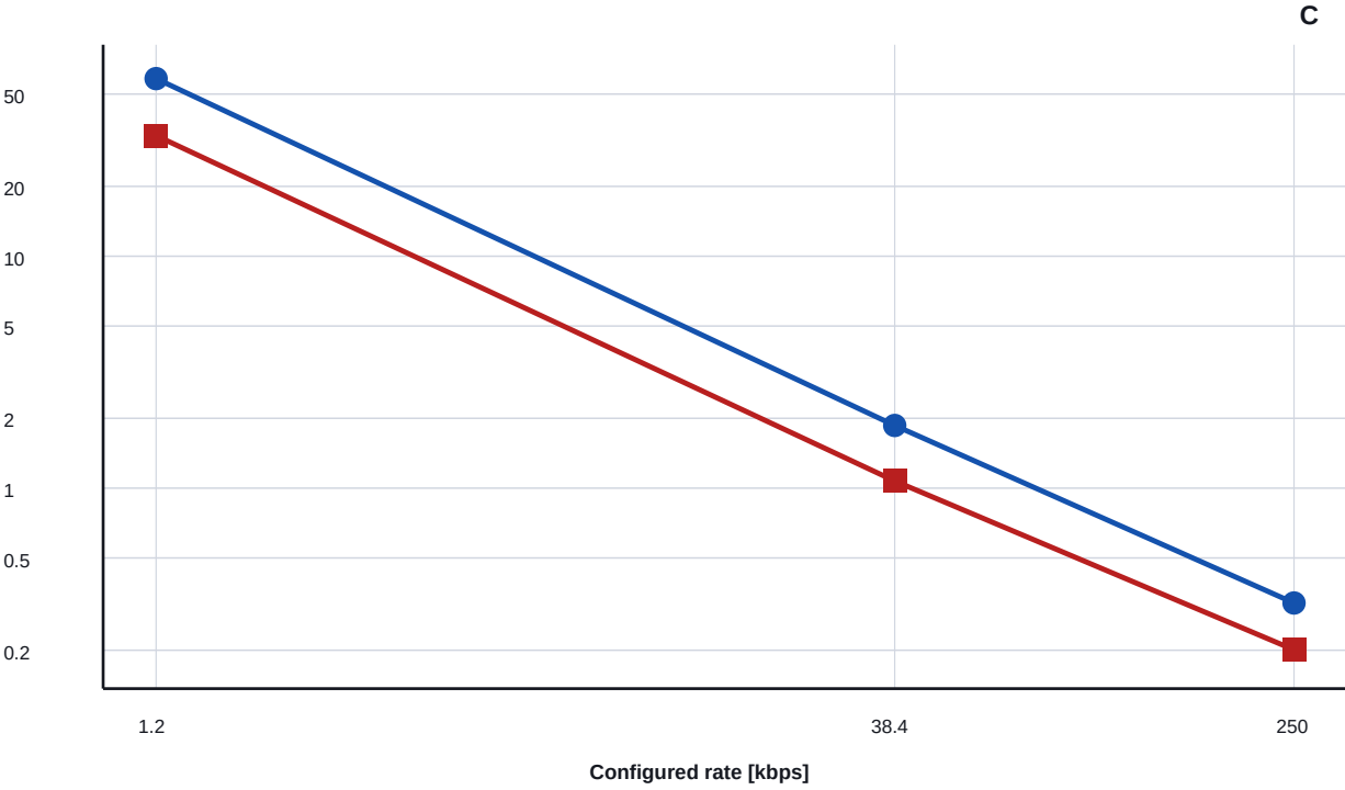
TX energy versus rate
