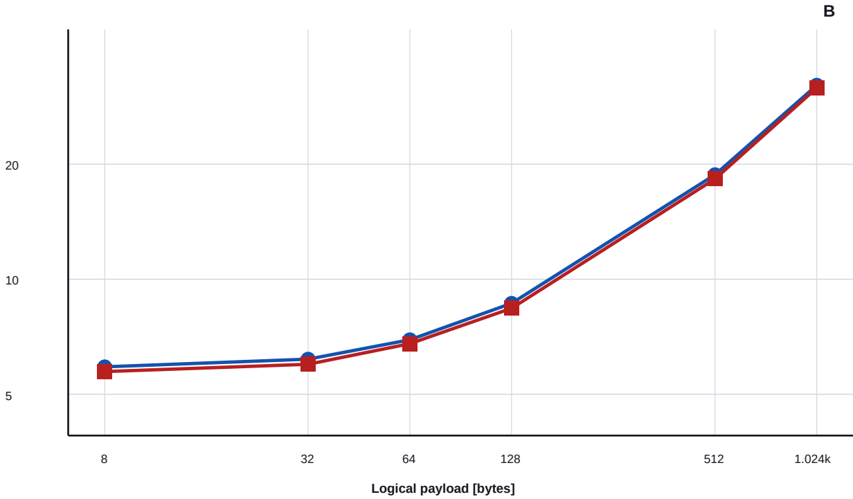
RX energy versus payload
