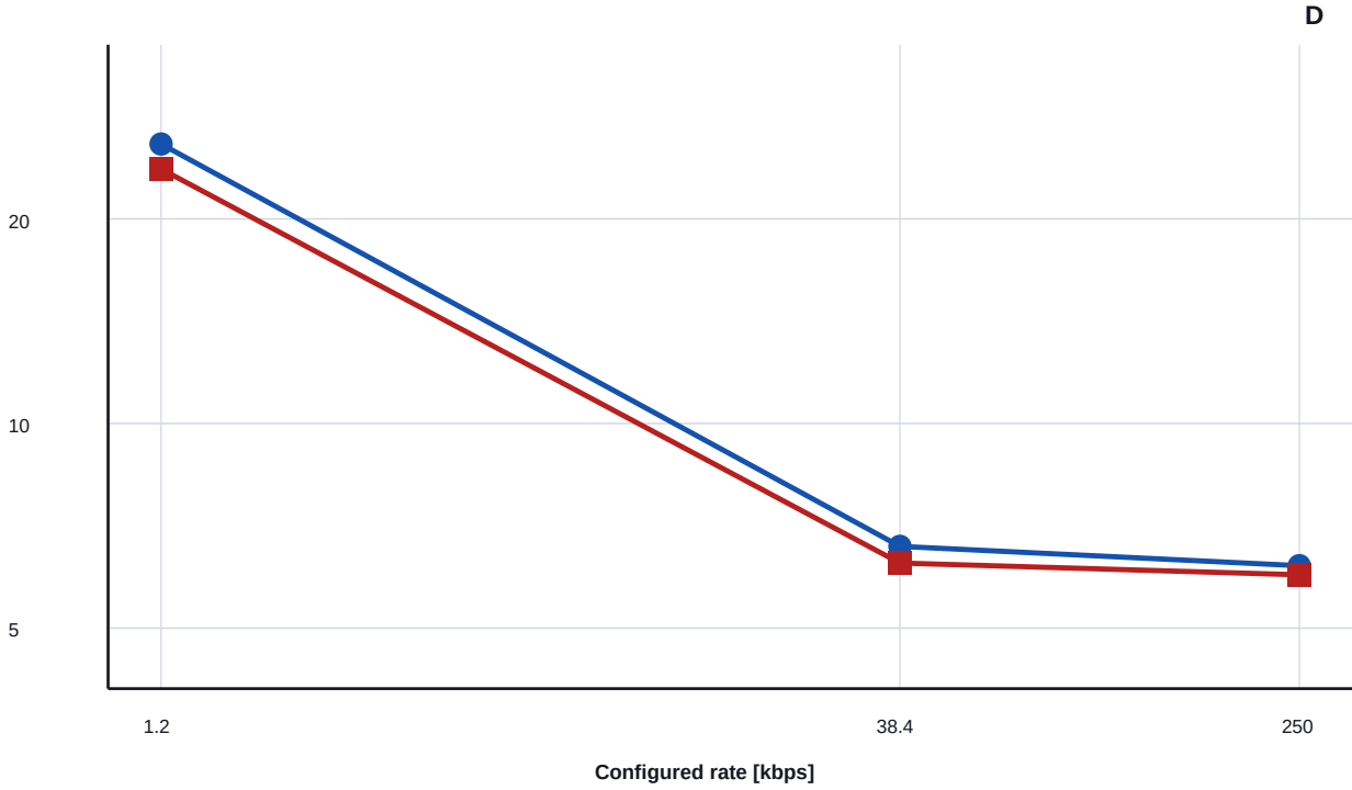
RX energy versus rate
