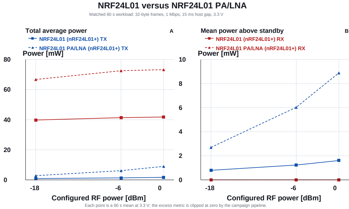
Figure 21: Matched NRF24L01 (nRF24L01+) continuous-power comparison at 1 Mbps. NRF24L01 PA/LNA (nRF24L01+) increases both TX and RX module-boundary power across all three configured radio-drive settings.
