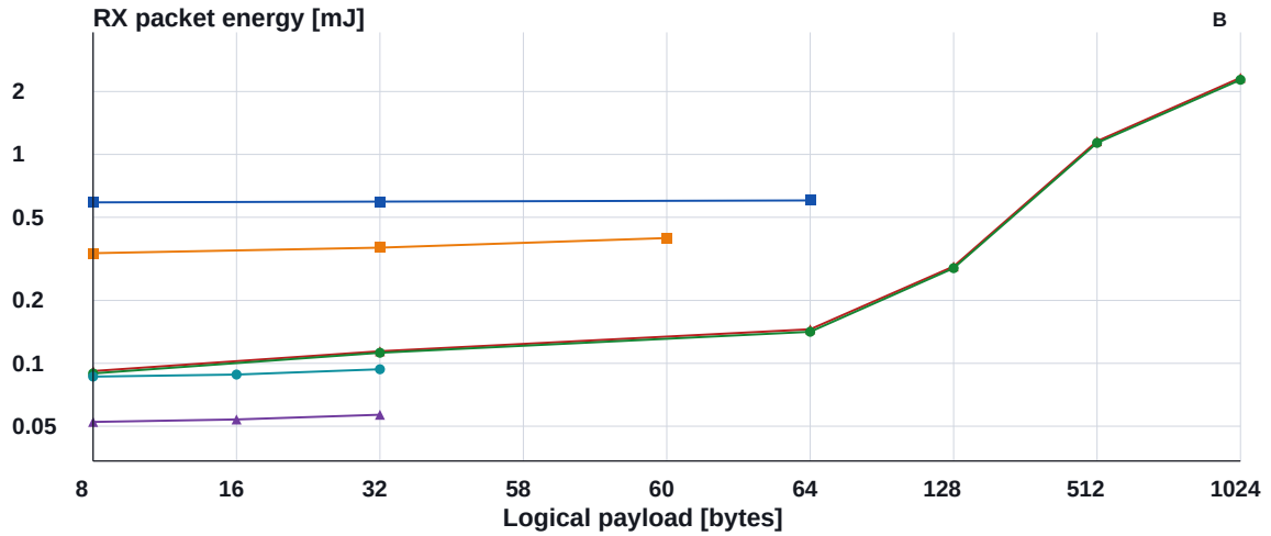
Figure 3: Measured RX event energy versus logical payload size, panels A–B, under the same per-module mode and configured-power rule as the TX matrix.
