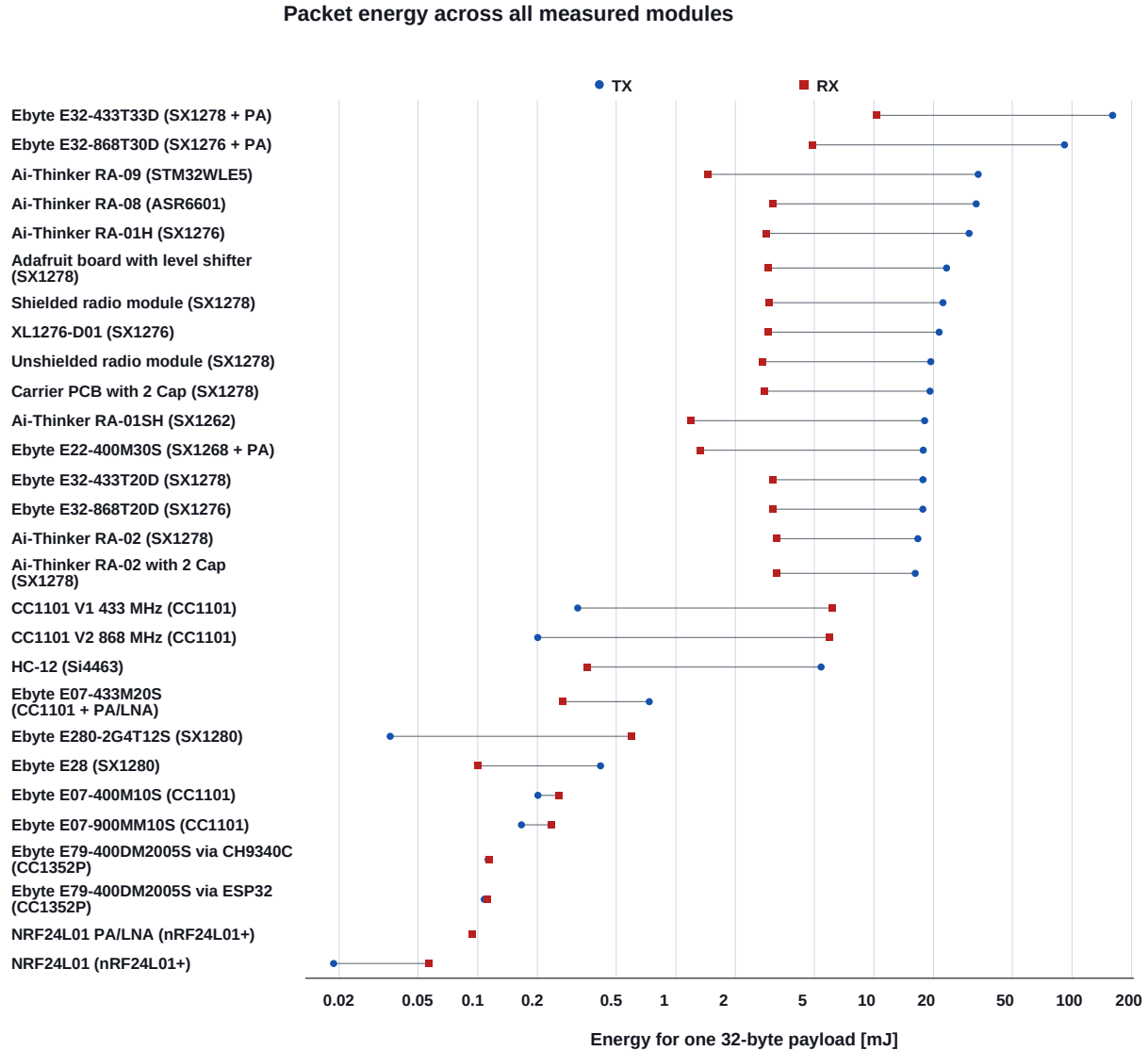
Figure 1: Total TX and RX event energy for a common 32-byte application payload. Logarithmic scaling is necessary because both air rate and output stage vary widely.
