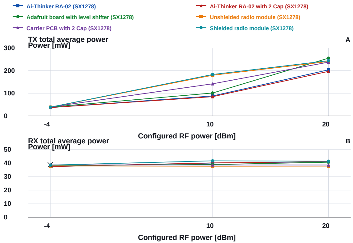
Figure 17: Matched continuous total-power comparison for all six SX1278 implementations from Figure 16. The TX and RX panels use independent vertical scales so that board-level differences remain visible.
