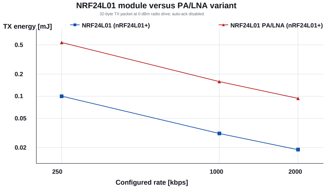
Figure 20: NRF24L01 (nRF24L01+) packet TX energy versus rate with and without the module-level PA/LNA. Both use the same 0 dBm radio-drive command.
