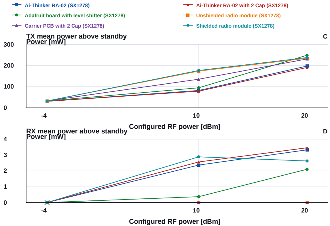
Figure 17: Matched continuous-power comparison for all six SX1278 implementations (continued): standby-subtracted TX and RX power. A black cross marks the Carrier PCB with 2 Cap (SX1278) RX window at -4 dBm, whose power trace is valid but whose receiver-delivery telemetry is missing.
