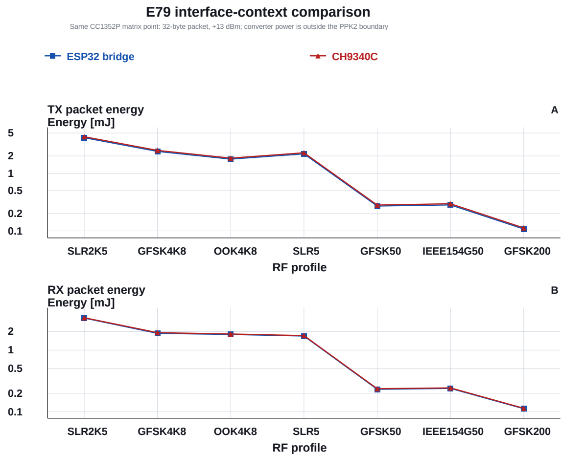
Figure 8: E79 packet energy measured through the original ESP32 UART bridge and the newer CH9340C path. The plotted 32-byte, +13-dBm points use identical PHY settings and modeled event durations. Bridge power is outside the PPK2 boundary.
