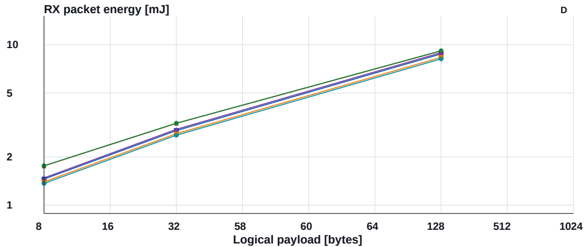
Figure 3: Measured RX event energy versus logical payload size, panels C–D (continued).
