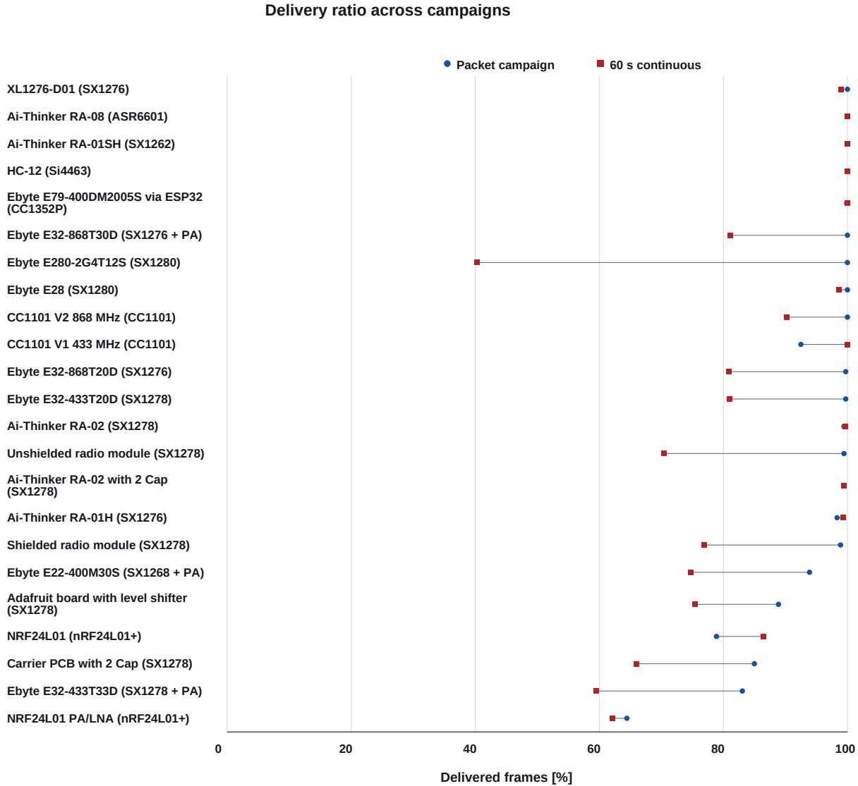
Figure 6: Aggregate packet and continuous delivery ratios for the 23 entries with both campaign types. The continuous ratio is an end-to-end bridge/modem/receiver result and is not a packet-error-rate sensitivity test.
