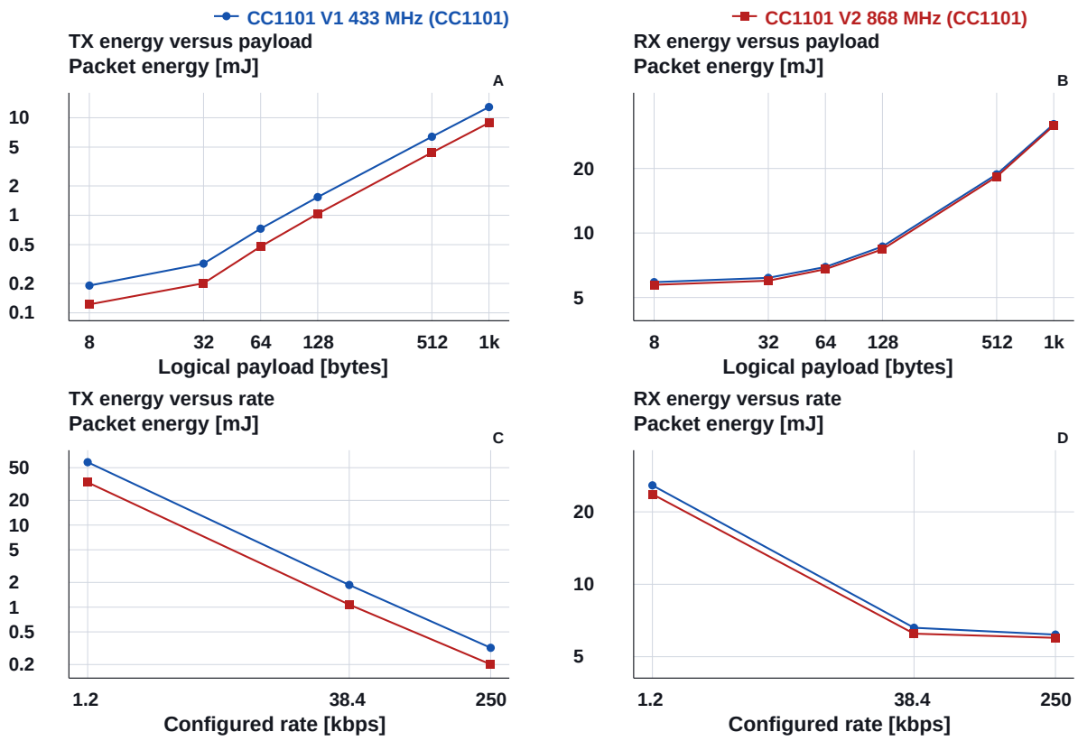
Figure 12: CC1101 packet-energy scaling on common axes. Payload panels use 250 kbps and +10 dBm; rate panels use a 32-byte payload and +10 dBm. Both axes are logarithmic.
