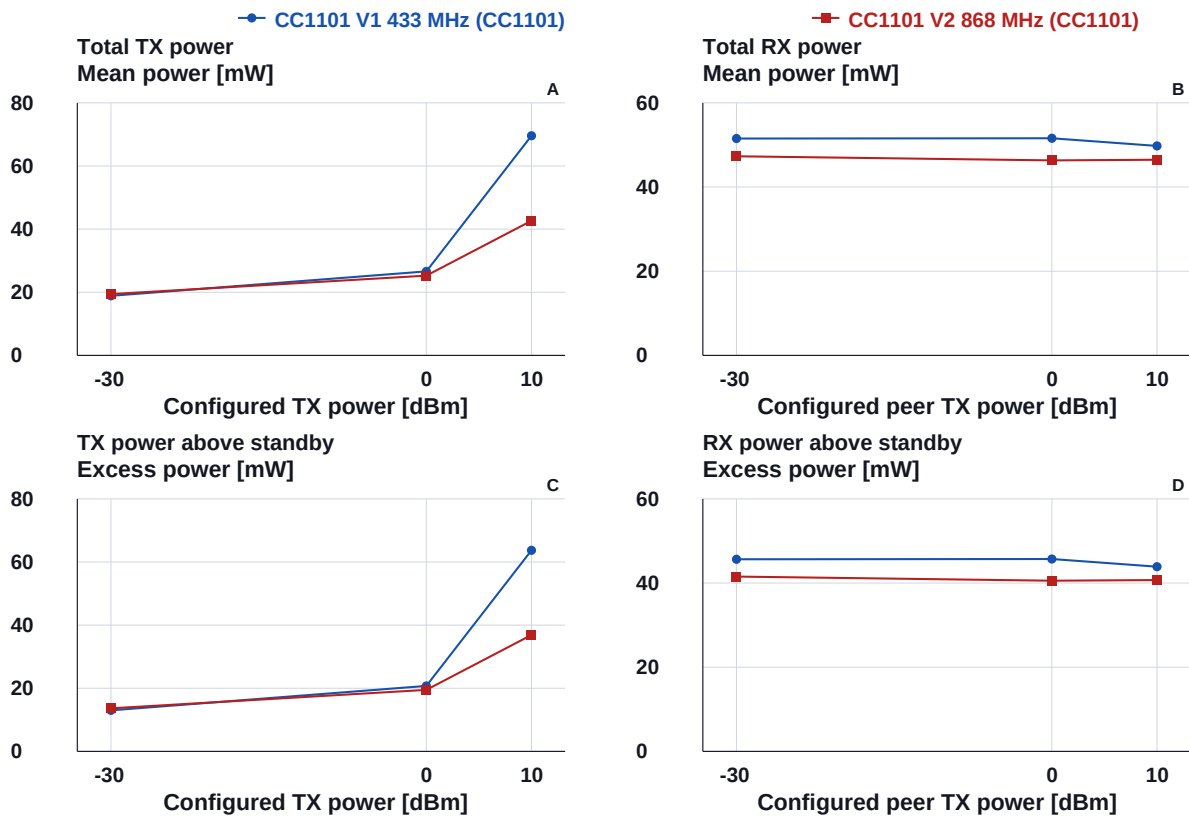
Figure 11: Controlled continuous-power comparison of the CC1101 V1 433-MHz and V2 868-MHz boards. Total and standby-subtracted values use the same 60-second, 32-byte, 38.4 kbps workload. The configured power on RX is the peer transmitter setting.
