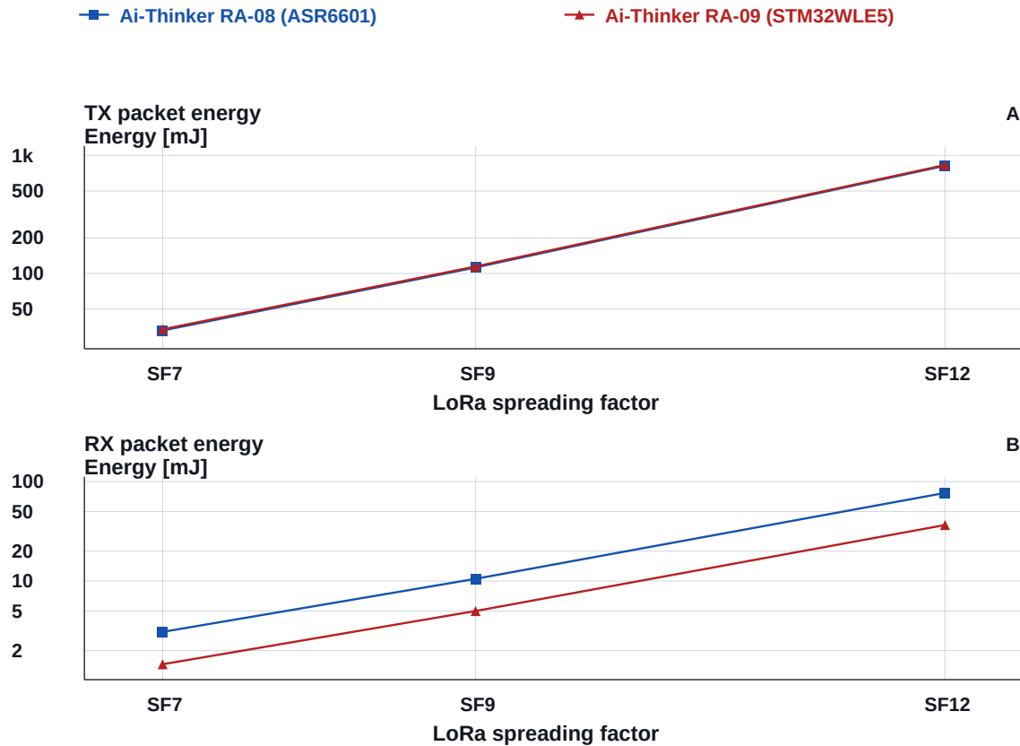
Figure 15: Matched Ai-Thinker RA-08 (ASR6601) and Ai-Thinker RA-09 (STM32WLE5) packet energy versus spreading factor for a 32-byte payload at BW125/CR4/5 and +22 dBm.
