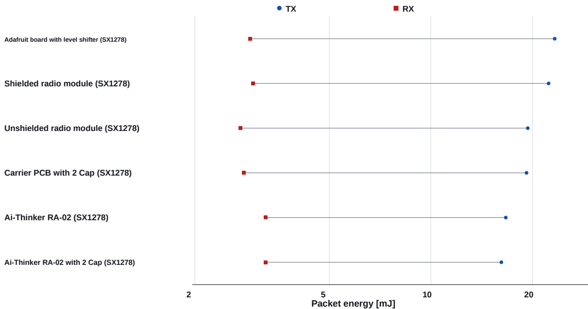
Figure 16: Controlled SX1278 comparison at 32 bytes, SF7/BW125/CR4/5, and +20 dBm. The same radio settings do not produce identical board-level energy.
