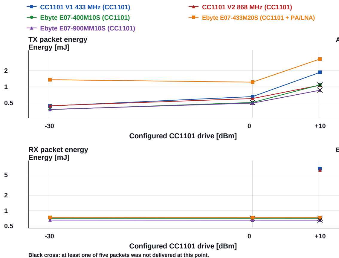
Figure 13: Module-boundary packet-energy comparison at a common 32-byte, 38.4 kbps GFSK/2-FSK workload. TX contains the full -30/0/+10 -dBm sweep for all five implementations. The legacy CC1101 RX campaigns contain only +10 -dBm peer points. A black cross marks an E07 point with incomplete delivery.
