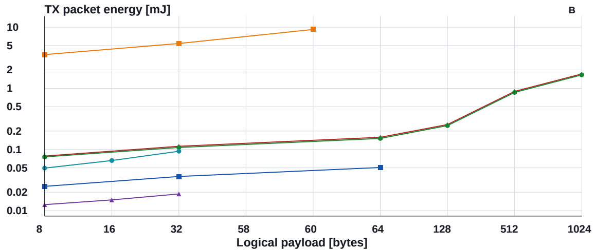
Figure 2: Measured TX event energy versus logical payload size, panels A–B. Lines connect measured points only; absent sizes are not interpolated in the numerical tables. Energy uses a logarithmic axis independently in each panel.
