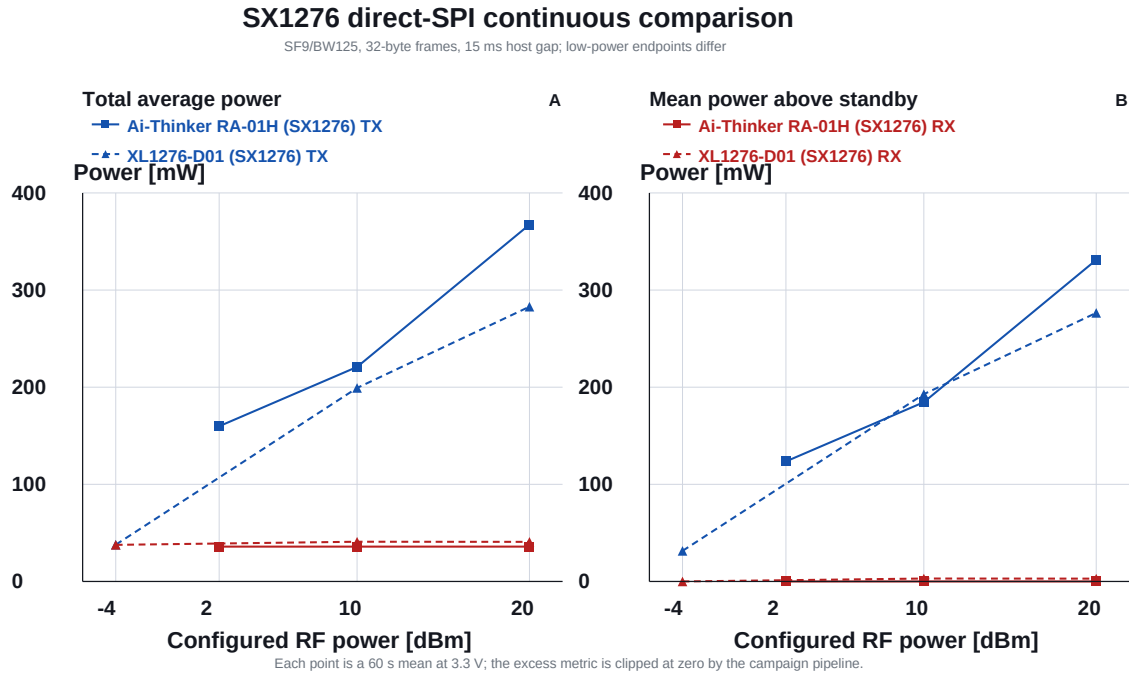
Figure 19: Controlled continuous-power comparison of the direct-SPI SX1276 subset, RA-01H and XL1276-D01, at SF9/BW125. Both include +10 and +20 dBm; the low endpoint is +2 dBm for RA-01H and -4 dBm for XL1276-D01.
