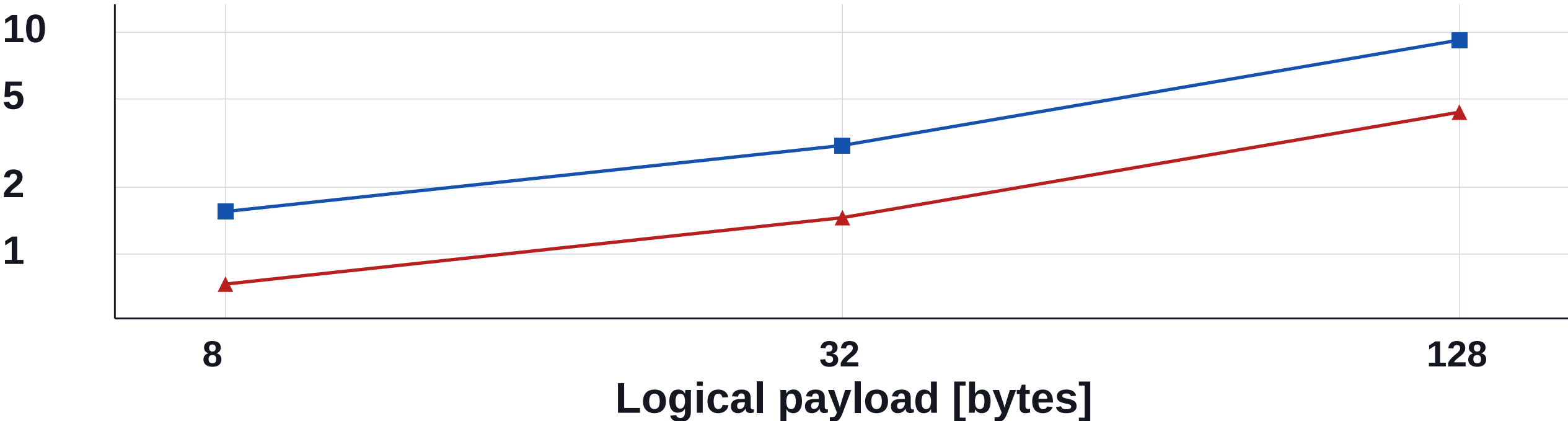
RX packet energy [mJ]
