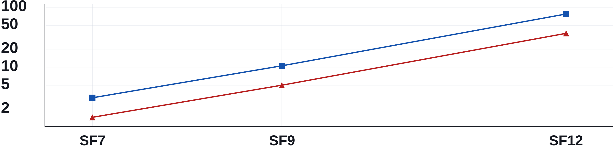
RX packet energy [mJ]
