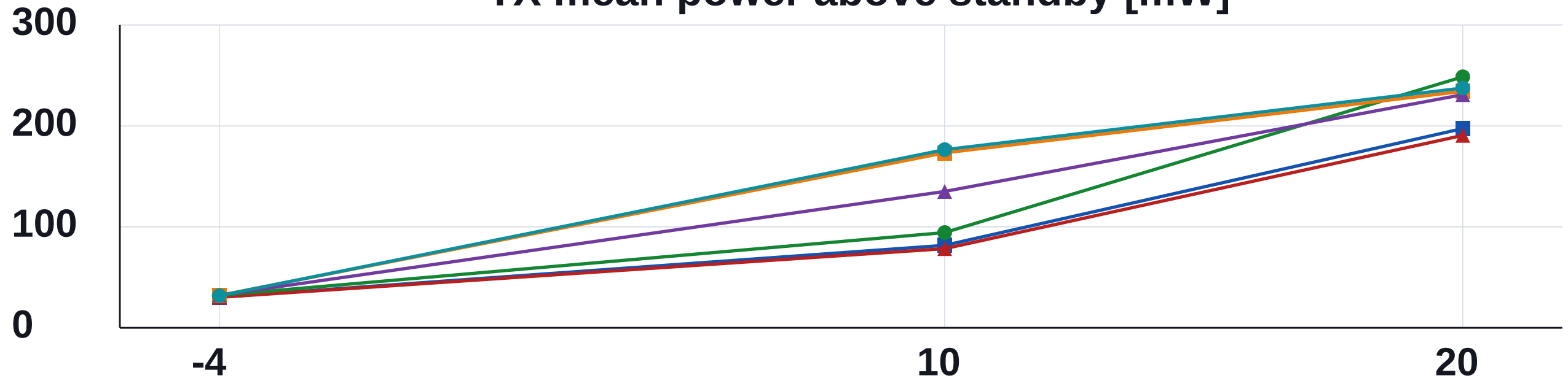
TX mean power above standby [mW]
