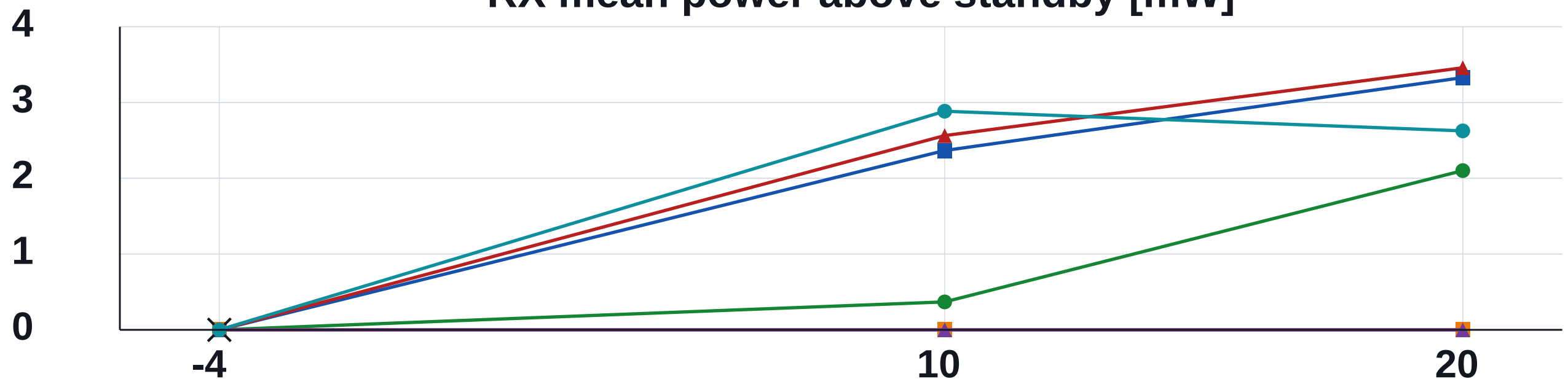
RX mean power above standby [mW]
