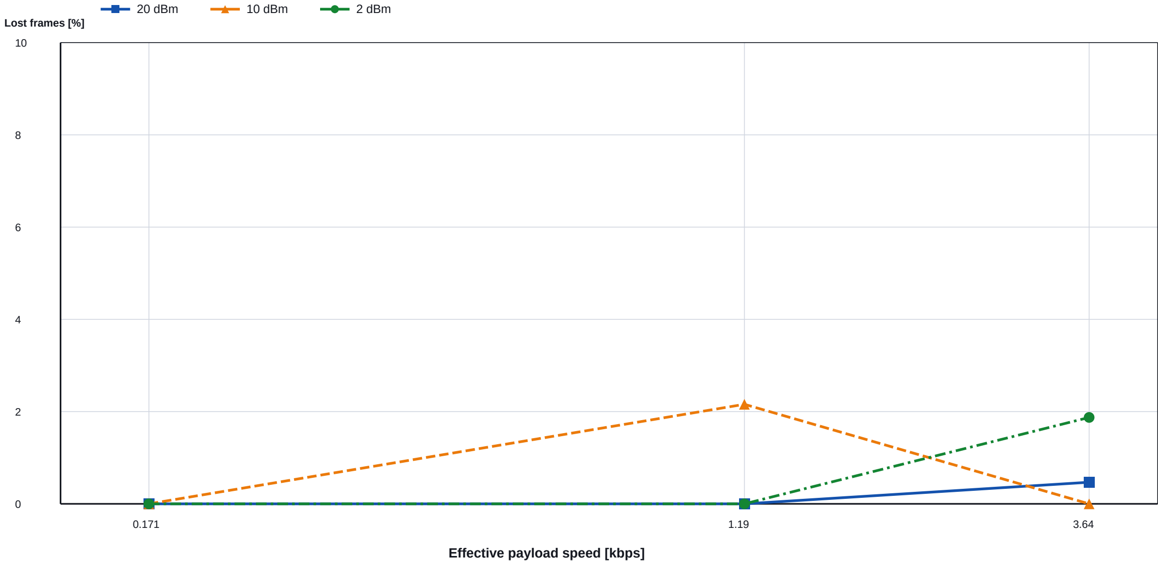
Ai-Thinker RA-01H (SX1276): loss versus effective payload speed
