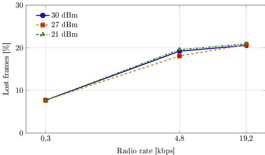
Ebyte E32-868T30D UART: packet loss versus radio rate
