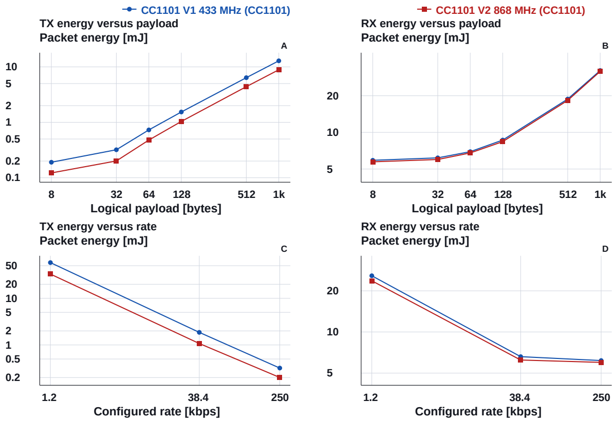
Figure 12: CC1101 packet-energy scaling on common axes. Payload panels use 250 kbps and +10 dBm; rate panels use a 32-byte payload and +10 dBm. Both axes are logarithmic.
