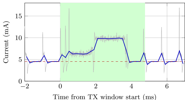
RX repetition 1: trigger vicinity
