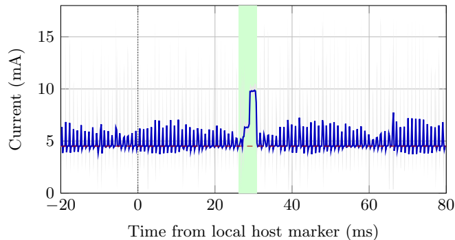
TX repetition 3: window detail
