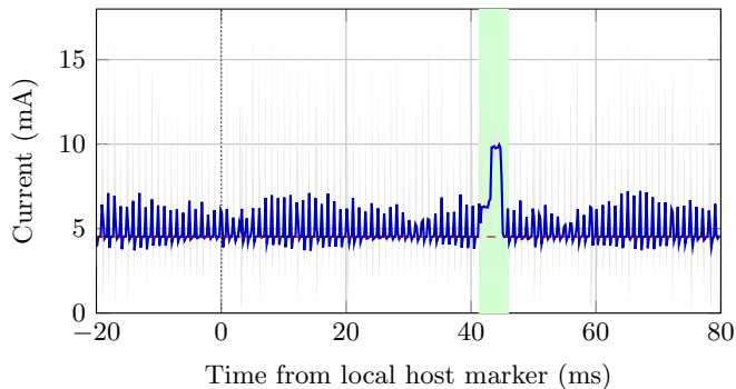
TX repetition 1: window detail
