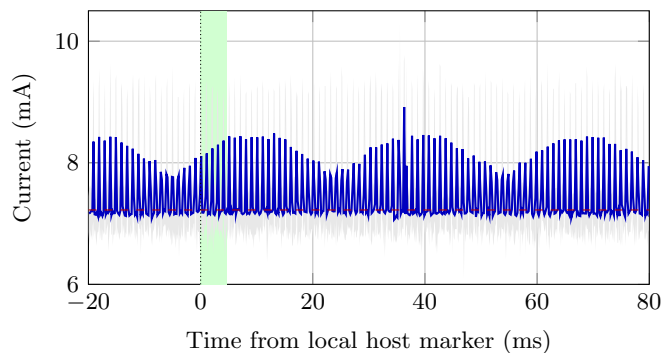
RX repetition 3: trigger vicinity
