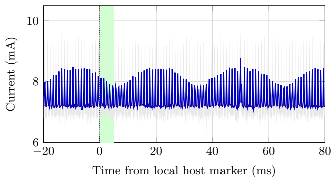
RX repetition 1: trigger vicinity
