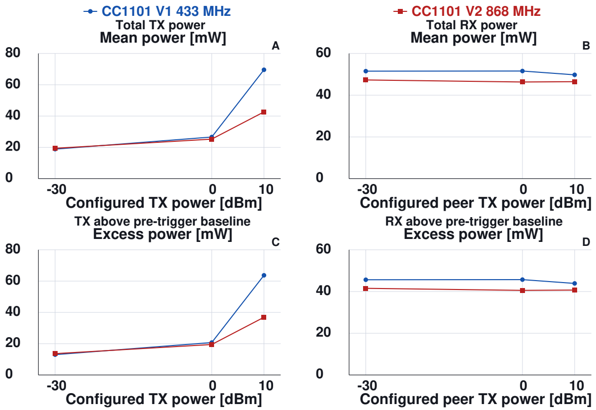
Figure 11: Controlled continuous-power comparison of the CC1101 V1 433-MHz and V2 868-MHz boards. Total and pre-trigger-baseline-subtracted values use the same 60-second, 32-byte, 38.4 kbps workload. These original sessions take the baseline with RX off. The configured power on RX is the peer transmitter setting.
