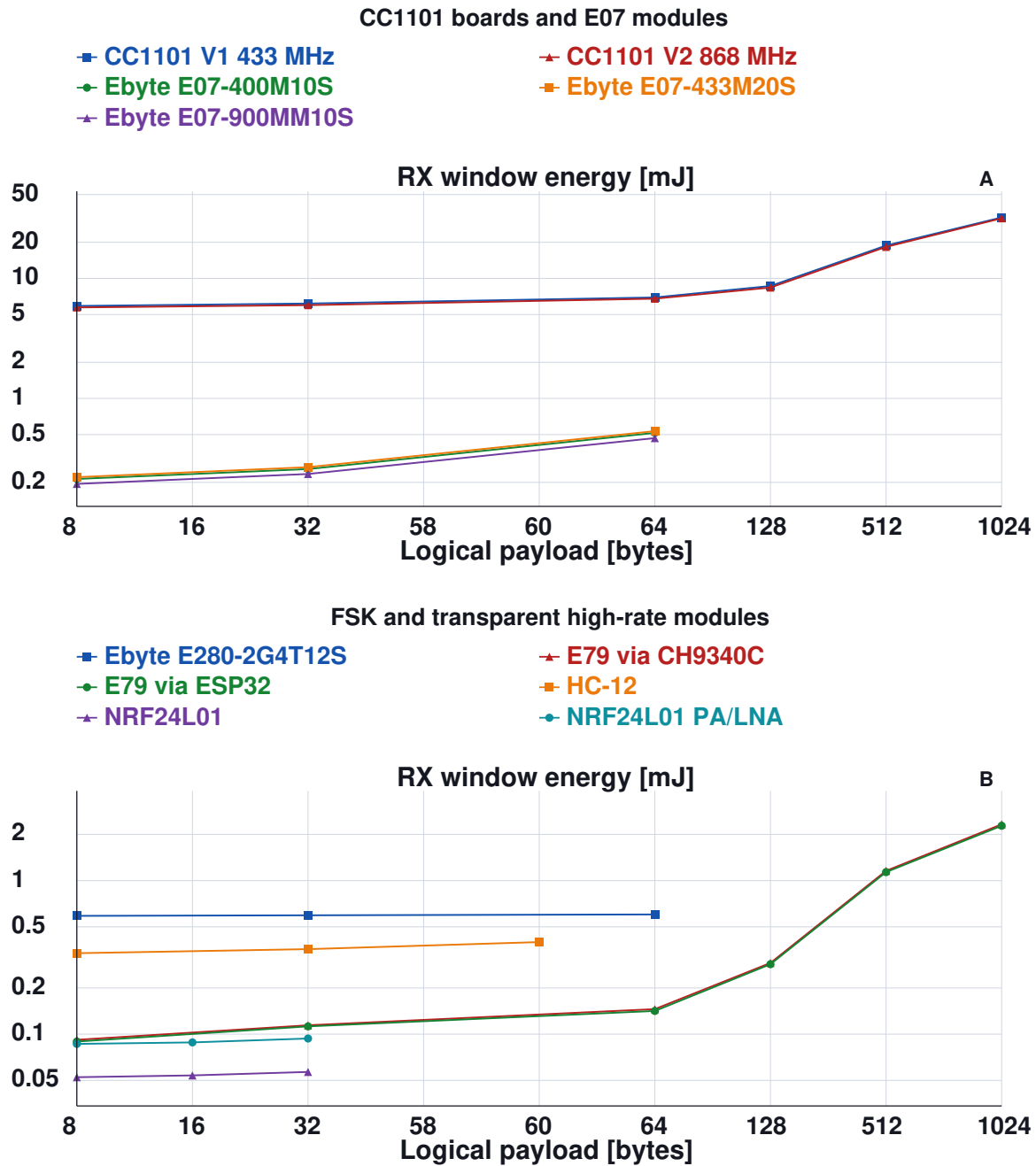
Figure 3: Measured RX integration-window energy versus logical payload size, panels A–B, under the same per-module mode and configured-power rule as the TX matrix.
