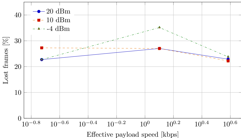
SX1278-Adafruit-LevelShifter: loss versus effective payload speed
