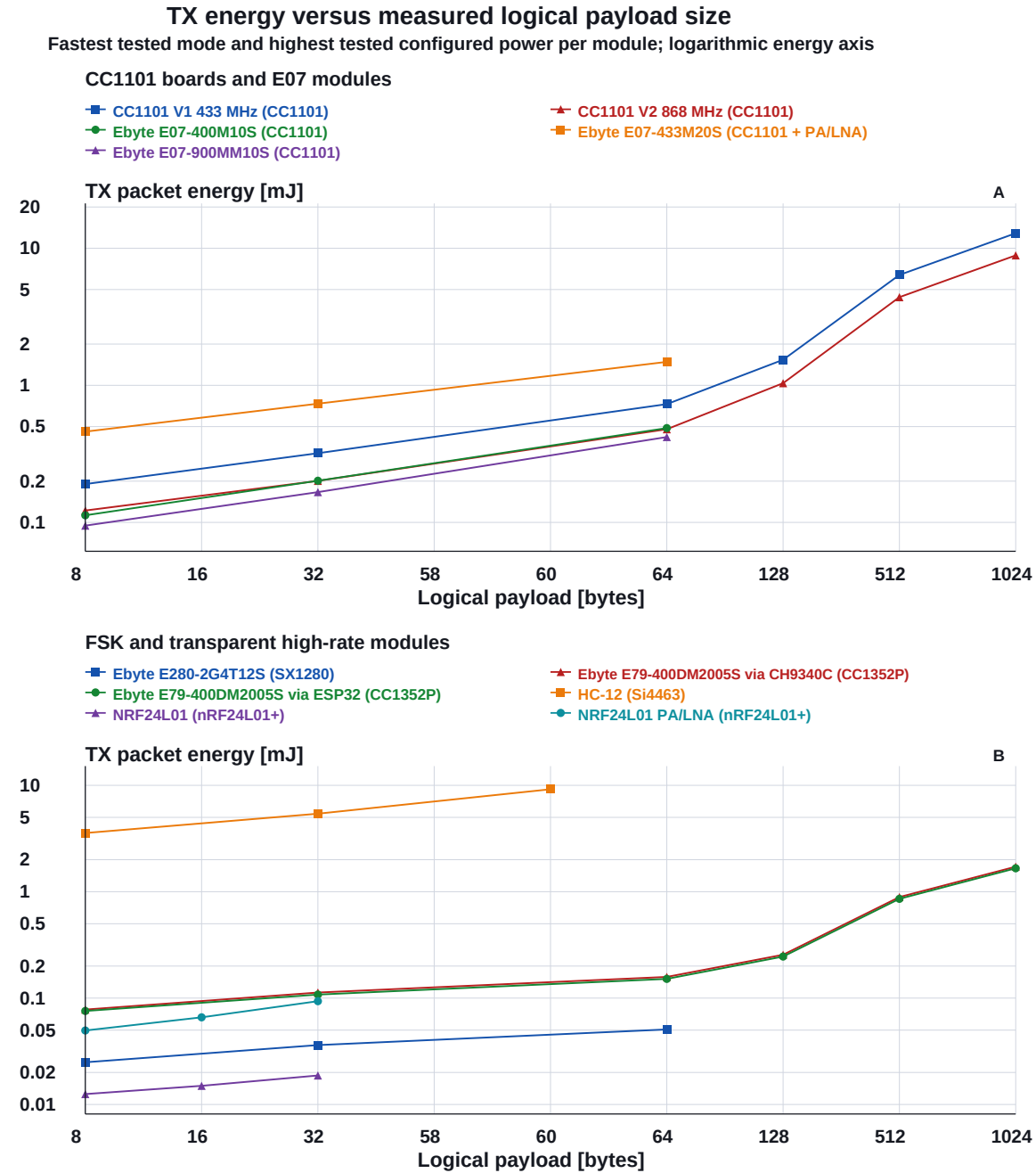
Figure 2: Measured TX event energy versus logical payload size, panels A–B. Lines connect measured points only; absent sizes are not interpolated in the numerical tables. Energy uses a logarithmic axis independently in each panel.
