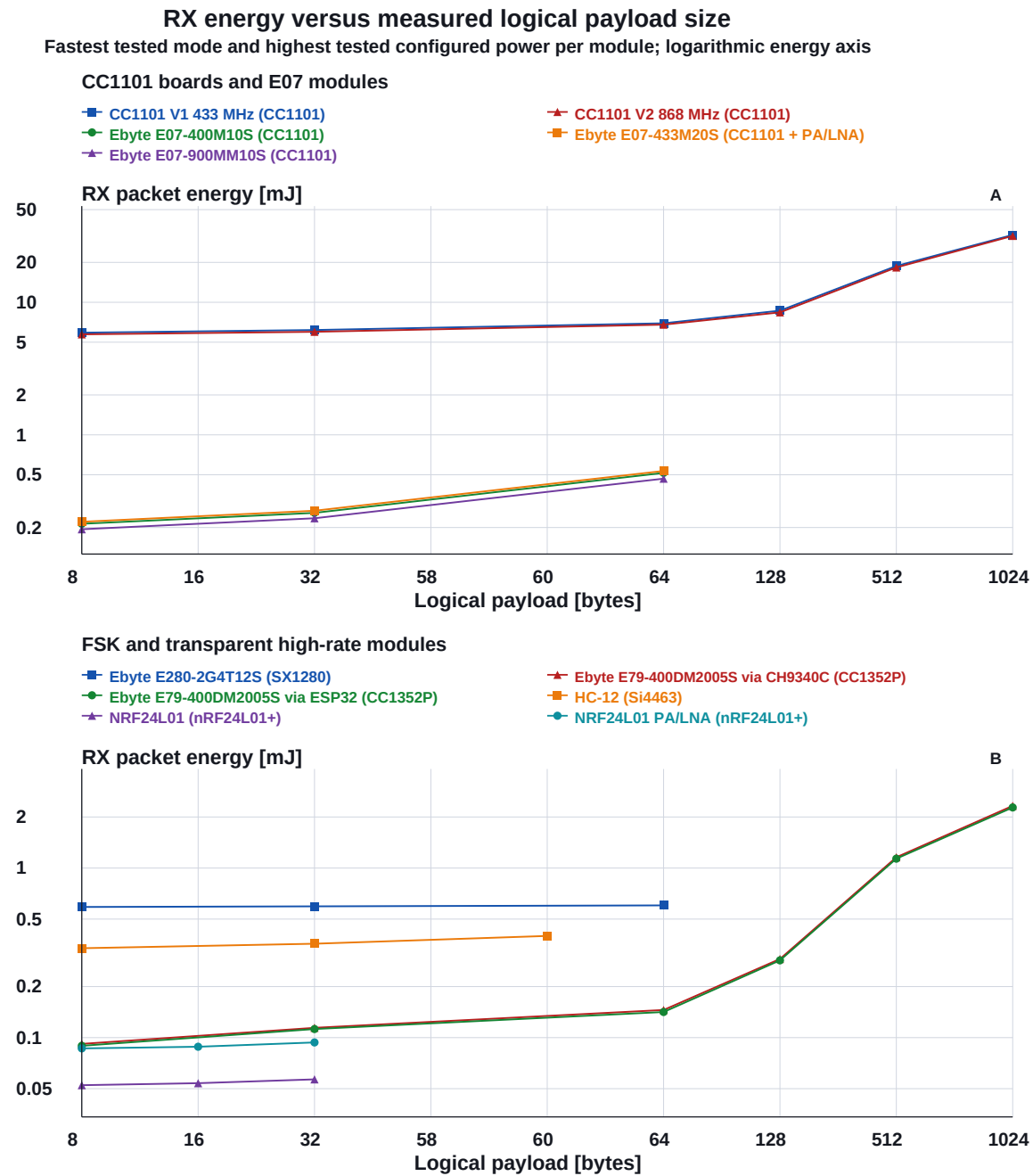
Figure 3: Measured RX event energy versus logical payload size, panels A–B, under the same per-module mode and configured-power rule as the TX matrix.
