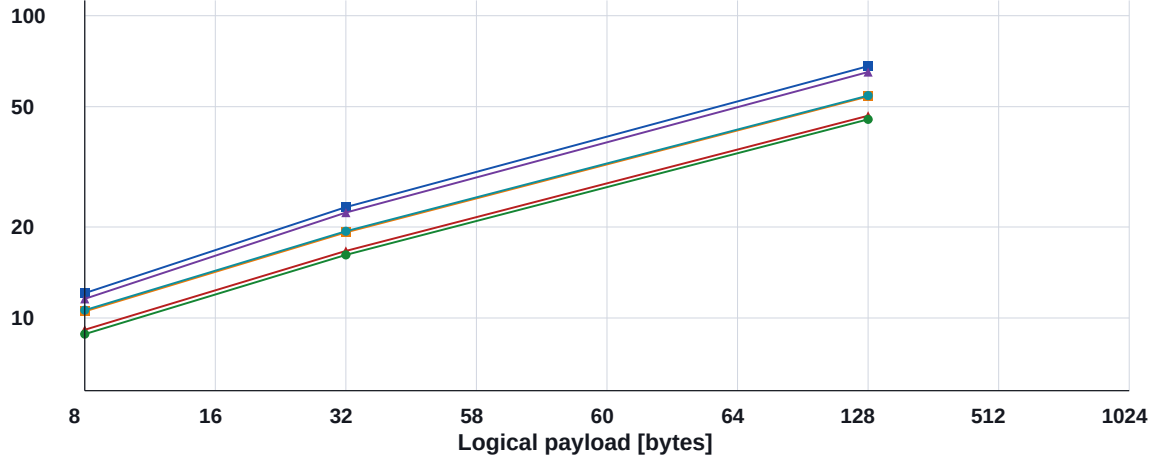
Figure 2: Measured TX event energy versus logical payload size, panels C–D (continued).
