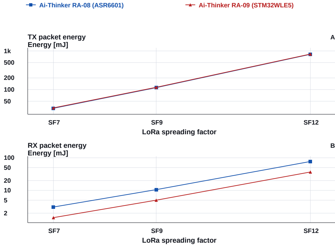
Ai-Thinker RA-08 (ASR6601) versus Ai-Thinker RA-09 (STM32WLE5): energy versus SF Matched 32-byte LoRa point at BW125/CR4/5 and +22 dBm
