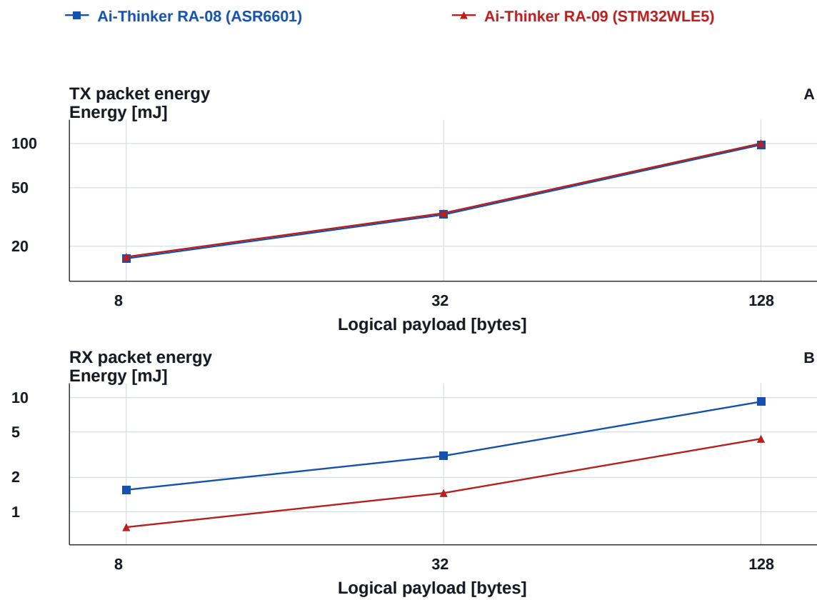
Ai-Thinker RA-08 (ASR6601) versus Ai-Thinker RA-09 (STM32WLE5): energy versus payload Matched LoRa point: SF7/BW125/CR4/5 and +22 dBm
