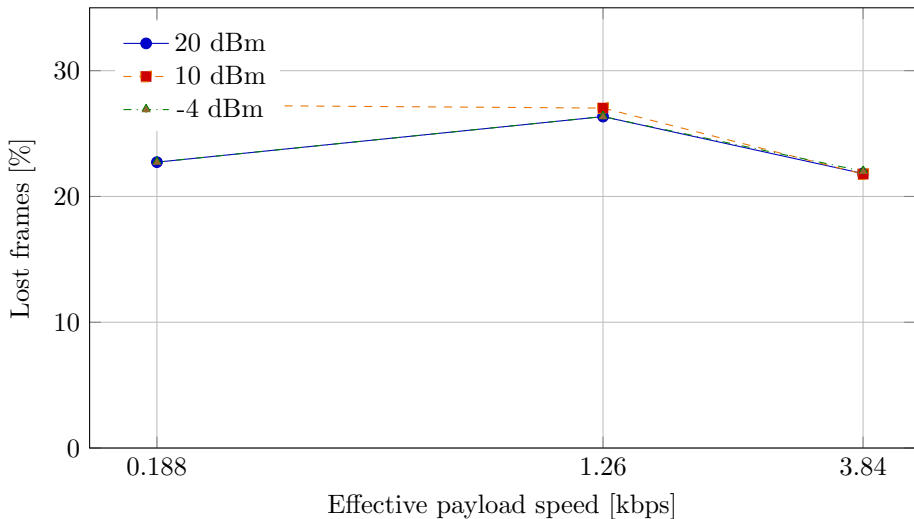
SX1278-Shielded: loss versus effective payload speed
