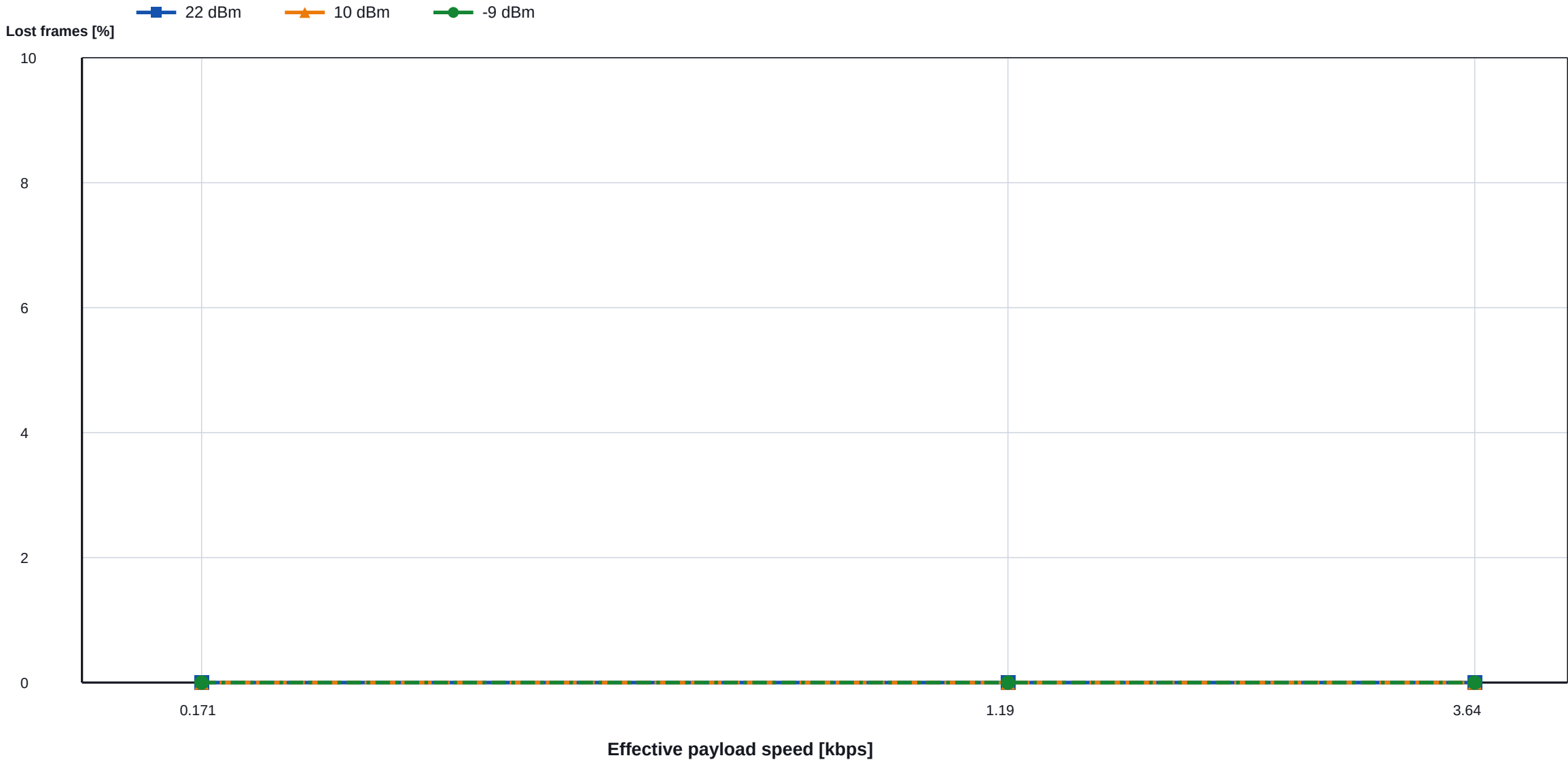
Ai-Thinker RA-01SH (SX1262): loss versus effective payload speed
