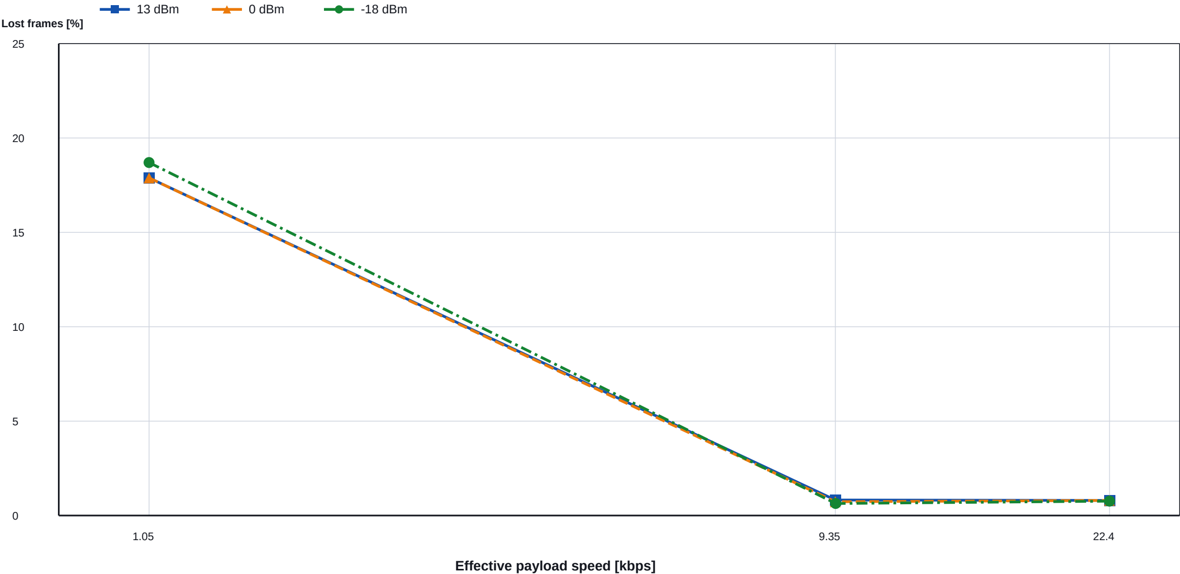
E28 direct SPI (SX1280): loss versus effective payload speed
