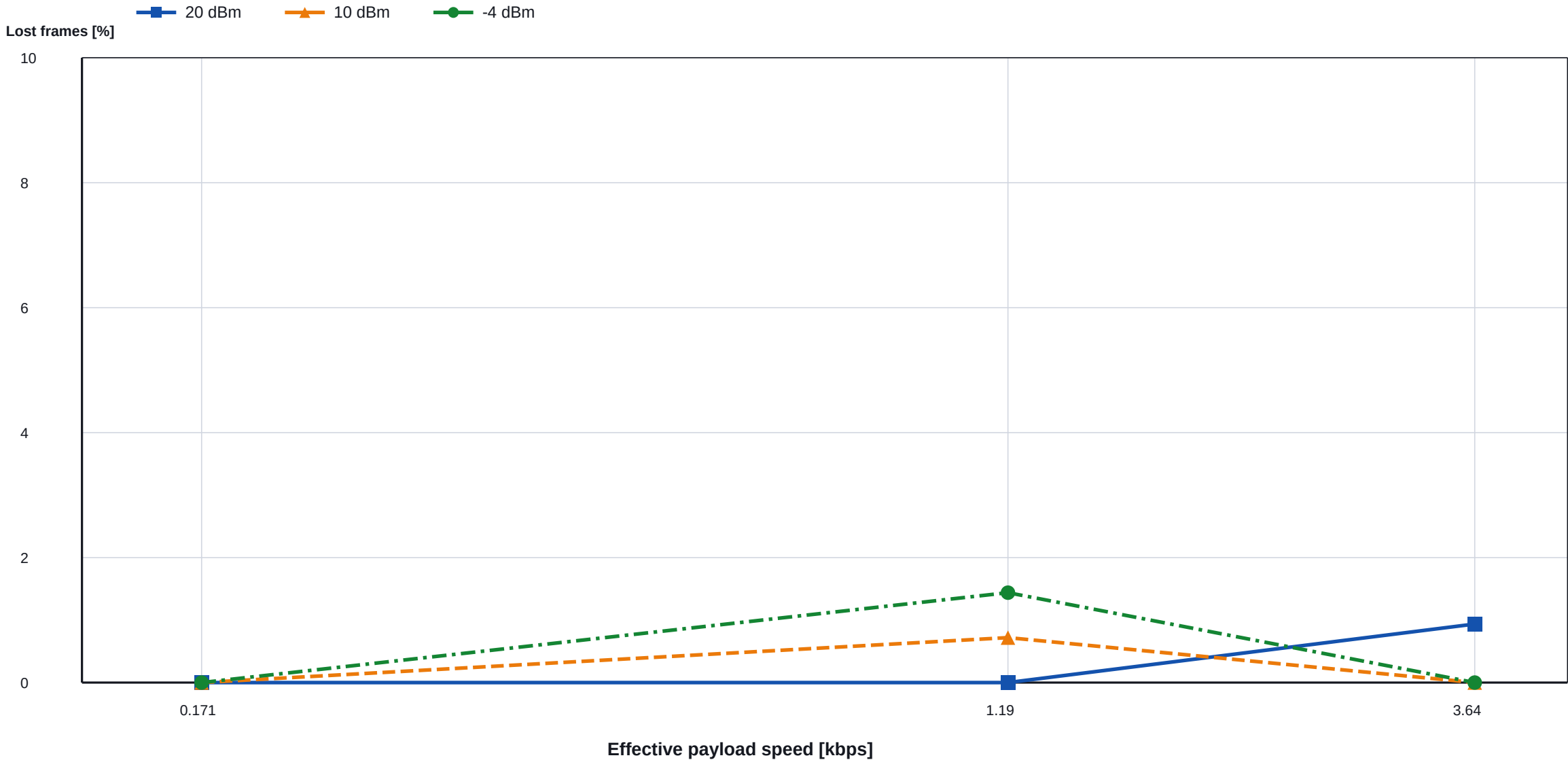
Ai-Thinker RA-02 (SX1278): loss versus effective payload speed
