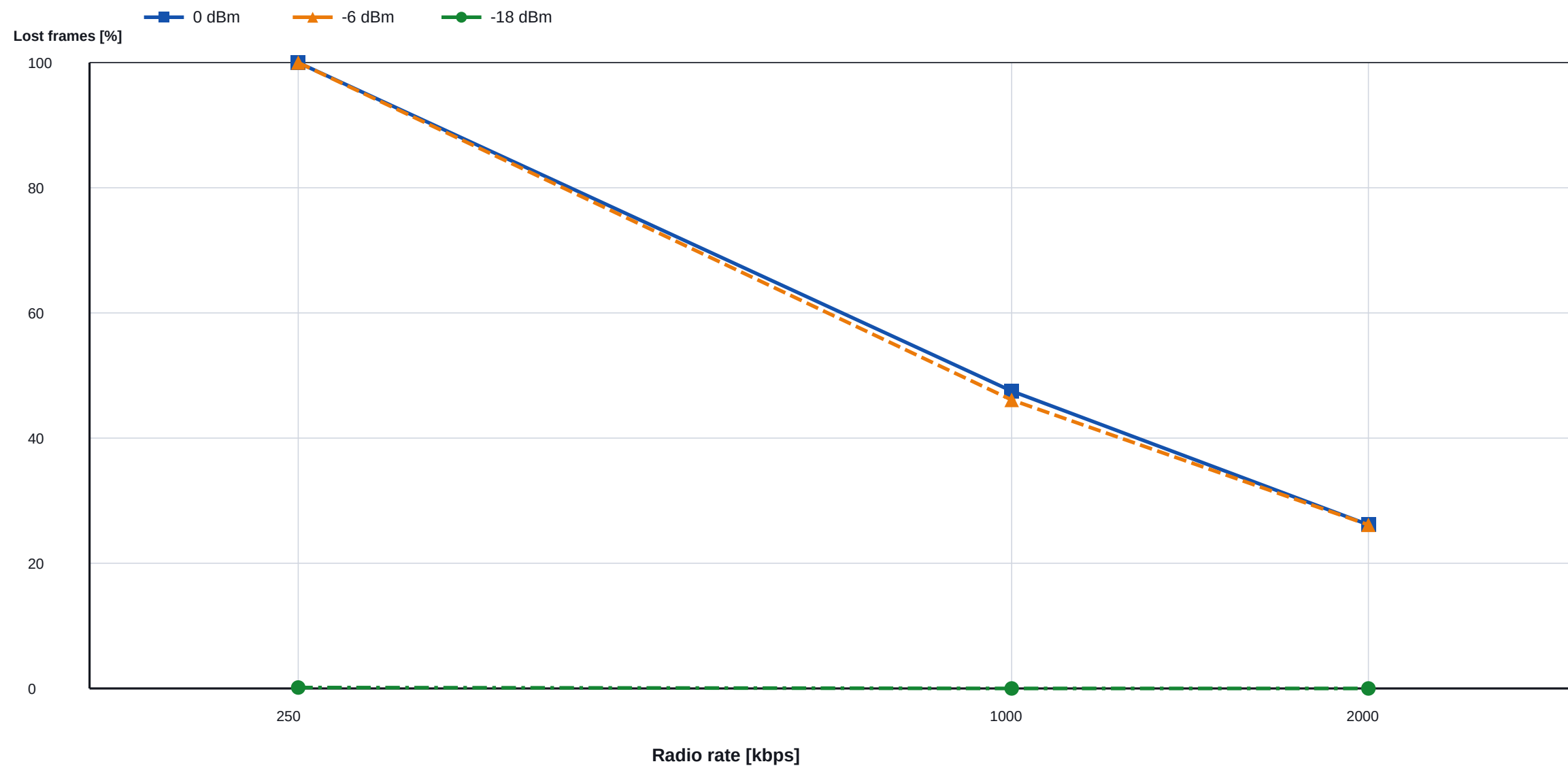
nRF24L01+PA: packet loss versus radio rate
