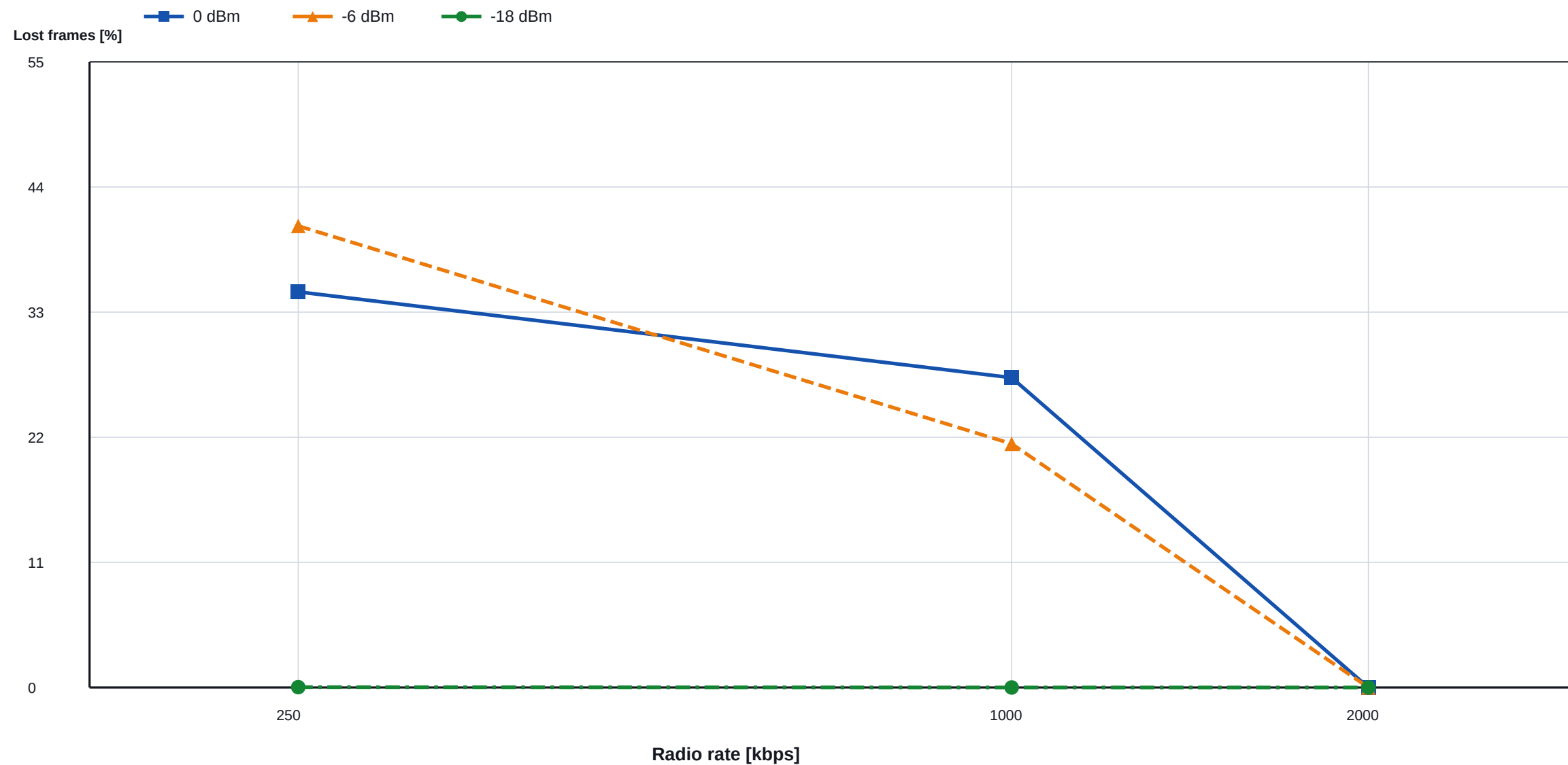
nRF24L01: packet loss versus radio rate
